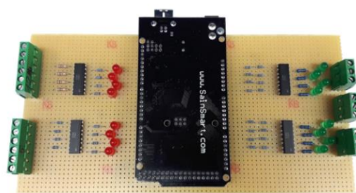
Figure 10. Completed test panel
