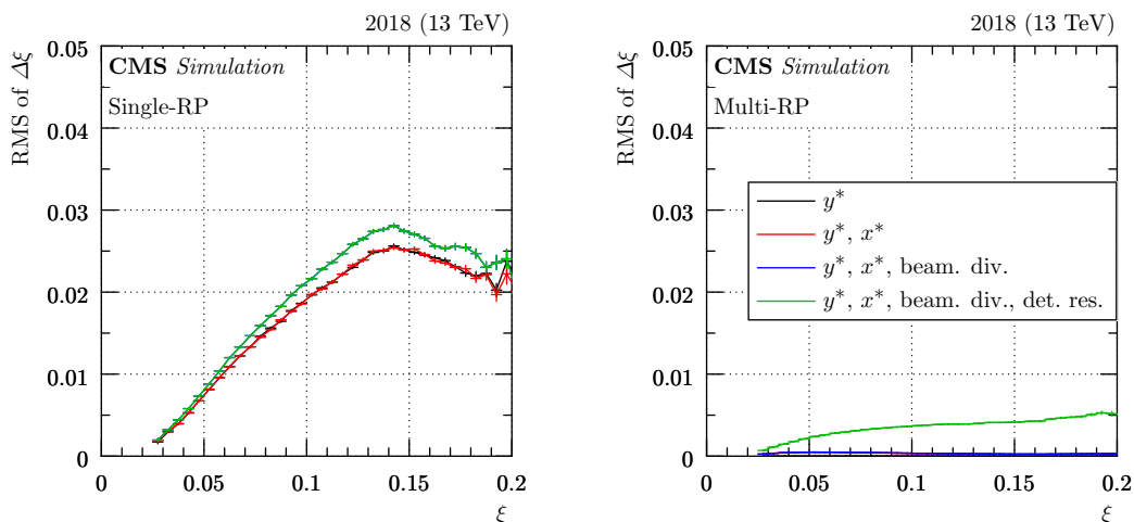
Figure 36. Example of resolution studies for \xi (2018 pre-TS1, sector 56). On the vertical axes, \Delta\xi refers to the difference between the reconstructed and simulated \xi . On the horizontal axes, \xi denotes the simulated value. The different colors refer to different smearing effects considered. Black: only vertical vertex smearing, red: in addition also horizontal vertex smearing, blue: in addition also beam divergence, green (the most complete scenario): in addition also detector spatial resolution. The error bars represent statistical uncertainties. Note that some curves are superimposed. Left: single-RP, right: multi-RP reconstruction.
