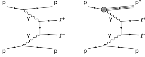
Figure 42. Diagrams for \gamma\gamma \rightarrow \mu^+\mu^- production with intact protons. Left: fully exclusive production, with both protons remaining intact. Right: Single proton dissociation, with one of the two protons remaining intact. In the right plot, the three lines labelled p^* indicate that the proton does not remain intact, but dissociates into an undetected low-mass system.
