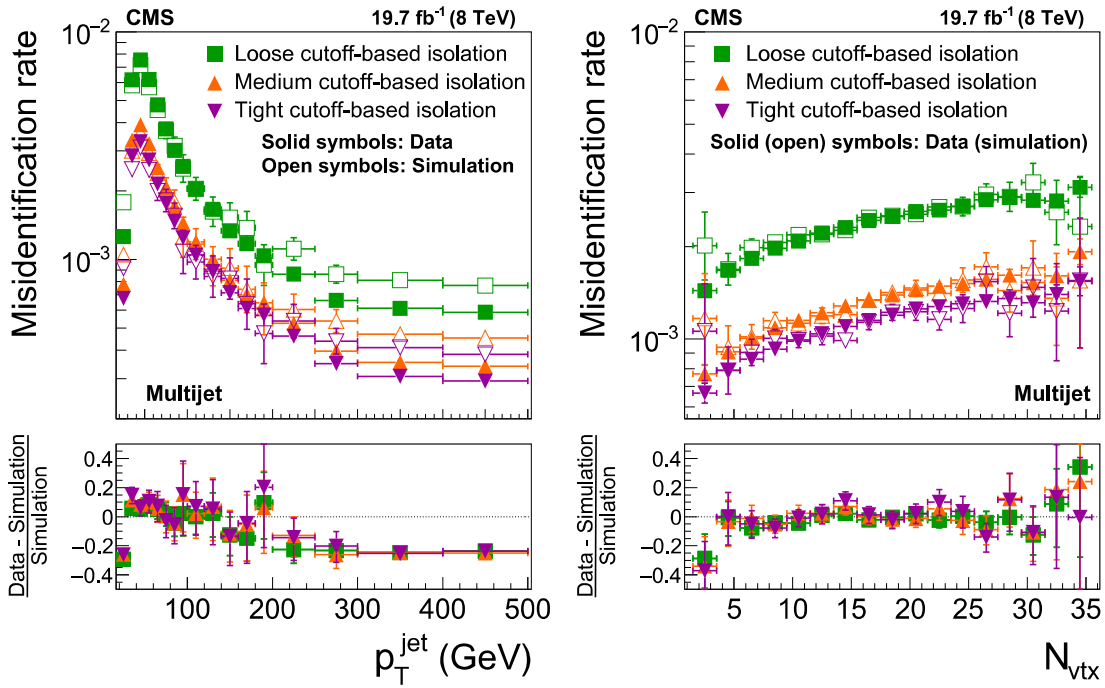
Figure 32. Probability for quark and gluon jets to pass the \tau_h reconstruction and \tau_h isolation criteria as a function of jet p_T (left) and number of reconstructed vertices (right) [52]. The misidentification rates measured in QCD multijet data are compared to the simulation.
