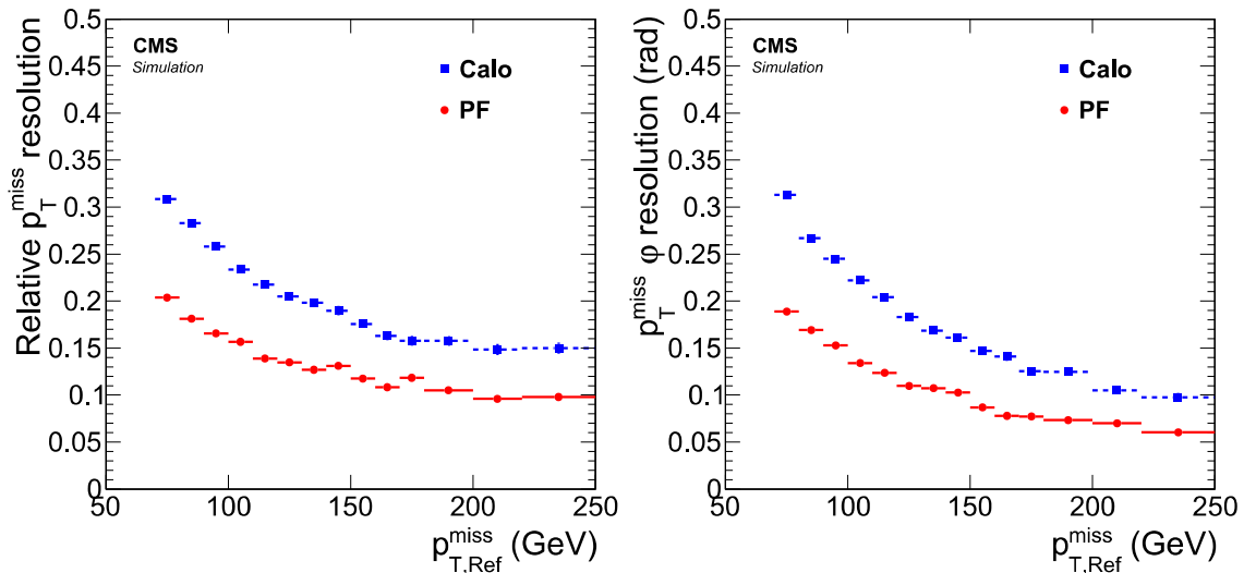
Figure 15. Relative p_T^{\text{miss}} resolution and resolution on the \vec{p}_T^{\text{miss}} direction as a function of p_{T,Ref}^{\text{miss}} for a simulated t\bar{t} sample.
