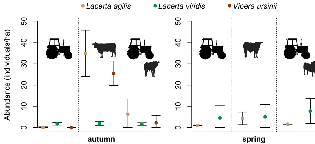
FIGURE 2 Abundance estimates (mean \pm 95% CI) of the study species on mowing, grazing, and mowing + grazing management sites by the two survey seasons analyzed.
