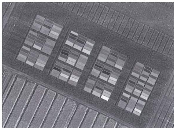
Figure 1: Measured SPAD values at the 6-leaf-stage of maize
