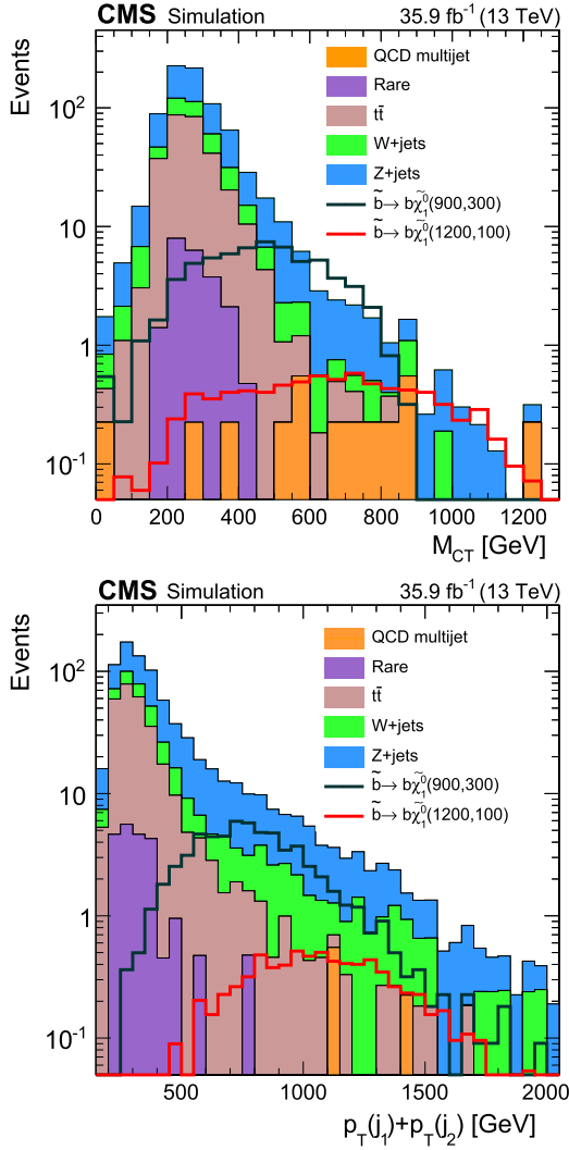
Fig. 2. Distribution of M_{CT} (upper) and p_{T(j_1)} + p_{T(j_2)} (lower) for the searches in noncompressed regions from simulation. The stacked, filled histograms represent different background components while the lines show two signal models with different bottom squark and neutralino mass hypotheses ( m_{\tilde{b}} = 900 GeV and m_{\tilde{\chi}_1^0} = 300 GeV) and ( m_{\tilde{b}} = 1200 GeV and m_{\tilde{\chi}_1^0} = 100 GeV). (For interpretation of the references to colour in this figure, the reader is referred to the web version of this article.)
