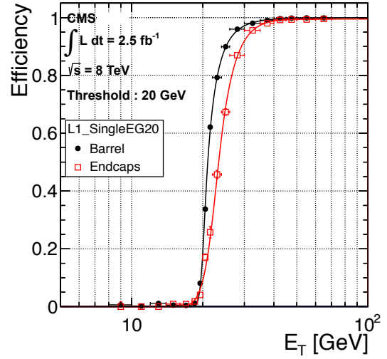
Figure 15. Electron trigger efficiency at L1 as a function of offline reconstructed E_T for electrons in the EB (black dots) and EE (red squares) using the 2012 data set (EG threshold: E_T = 20 GeV). The curves show unbinned likelihood fits.
