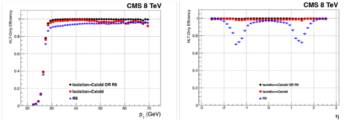
Figure 20. Efficiencies of the leading leg for the double-photon trigger as a function of the photon transverse energy (left) and pseudorapidity (right), as described in the text. The red symbols show the efficiency of the isolation plus calorimeter identification requirement, and the blue symbols show the efficiency of the R_9 selection criteria. The black symbols show the combined efficiency.
