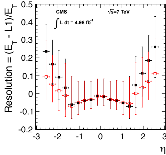
Figure 10. The L1 EG resolution for all electron p_T as a function of pseudorapidity \eta . For each \eta bin, a fit to a Crystal Ball function was used to model the data distribution. The vertical bars on each point represent the sigma of each fitted function which is defined as the width of the 68% area. The red points show the improved resolution after applying transparency corrections (as discussed in section 2.2.1).
