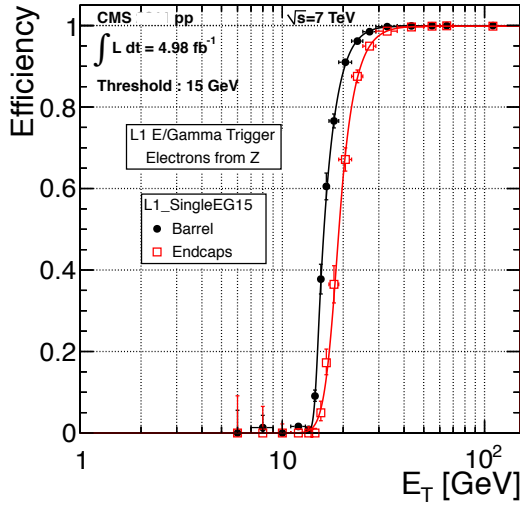
Figure 11. The electron trigger efficiency at L1 as a function of offline reconstructed E_T for electrons in the EB (black dots) and EE (red dots), with an EG threshold: E_T = 15 GeV. The curves show unbinned likelihood fits.
