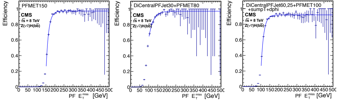
Figure 59. Trigger efficiencies for the Z(\nu\bar{\nu})H(b\bar{b}) analysis, as a function of offline PF E_T^{\text{miss}} for the pure E_T^{\text{miss}} > 150 GeV trigger (left) using late 2012 data, dijet and E_T^{\text{miss}} trigger (center) using early 2012 data, and dijet, E_T^{\text{miss}} and \Delta\phi requirement trigger (right) using 2012 late data, as described in the text.
