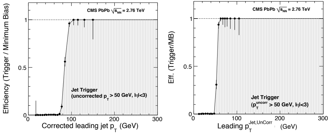
Figure 52. Efficiency curves for the Jet50U trigger in PbPb at \sqrt{s_{NN}} = 2.76 TeV, as a function of the corrected (left) and uncorrected (right) leading jet transverse momentum.
