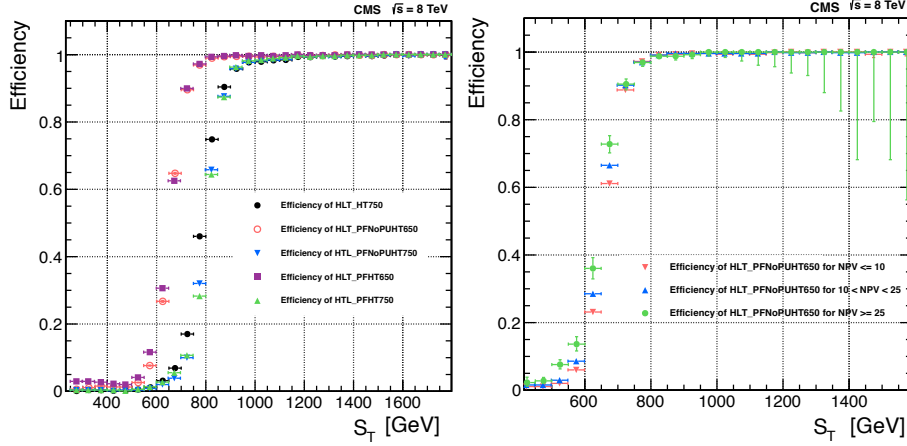
Figure 67. Left: efficiency of unscaled total jet activity HLT paths as a function of S_T . Right: efficiency of HLT_PFNPUHT650 as a function of S_T in three bins of number of primary vertices, N_{PV} : (i) N_{PV} \leq 10 , (ii) 10 < N_{PV} < 25 , and (iii) N_{PV} \geq 25 . All efficiencies are calculated with respect to a prescaled total activity path with H_T = 450 GeV threshold.
