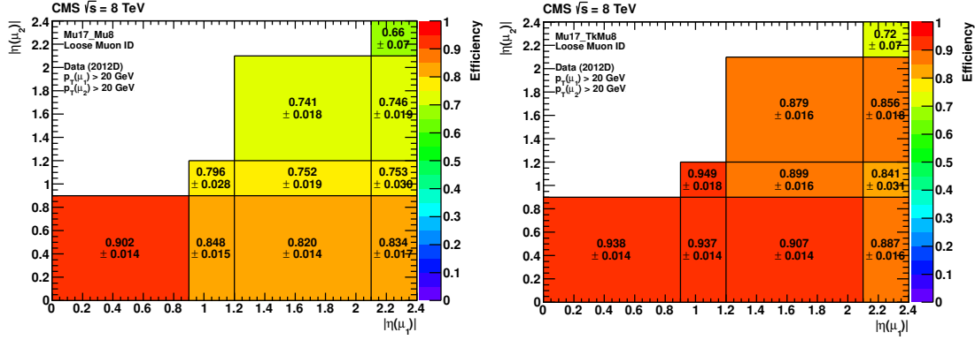
Figure 34. Efficiencies of double-muon triggers without (left) and with (right) the tracker muon requirement in 2012 data collected at 8 TeV as functions of the pseudorapidity |\eta| of the two muons, for loose muons with p_T > 20 GeV.
