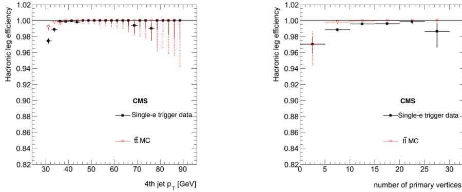
Figure 61. Top quark triggers: efficiency of the hadronic leg for the electron plus jets paths in 2012 as a function of the p_T of the 4th jet (left) and of the number of reconstructed vertices (right).
