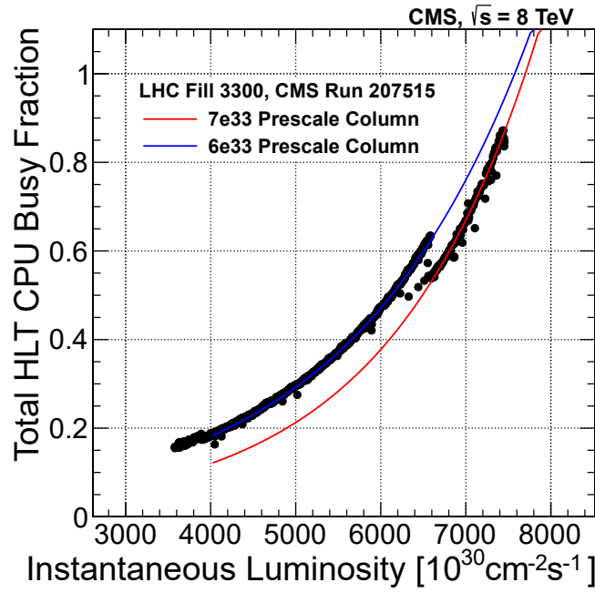
Figure 74. The average CPU busy fraction as a function of instantaneous luminosity for one LHC fill. Luminosity sections with data-taking downtime >40\% are removed.
