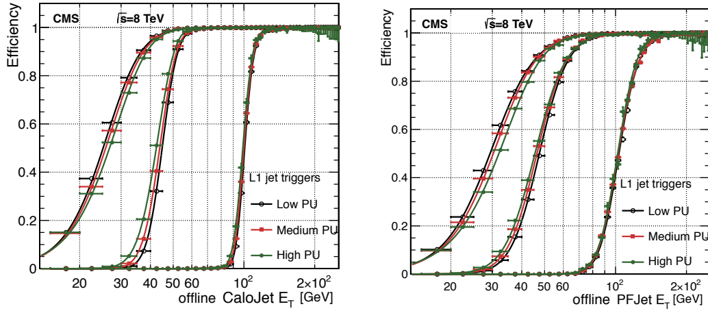
Figure 38. The L1 jet efficiency turn-on curves as a function of the leading offline CaloJet E_T (left) and as a function of the leading offline PF jet E_T (right), for low-, medium-, and high-pileup scenarios for three different thresholds: E_T > 16, 36 , and 92 GeV.
