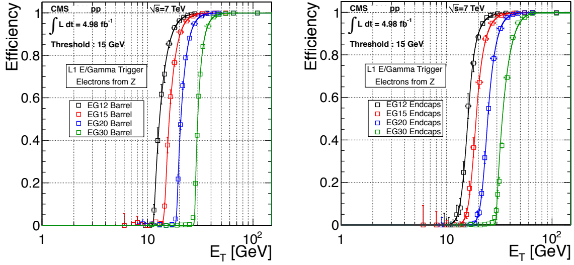
Figure 13. The L1 electron triggering efficiency as a function of the reconstructed offline electron E_T for barrel (left) and endcap (right). The efficiency is shown for the EG12, EG15, EG20 and EG30 L1 trigger algorithms. The curves show unbinned likelihood fits.
