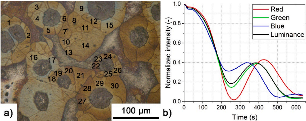
Fig. 13. Spheroidal graphite cast iron with the selected 30 ferrite grains (a) and the calculated average intensity curves (b).
