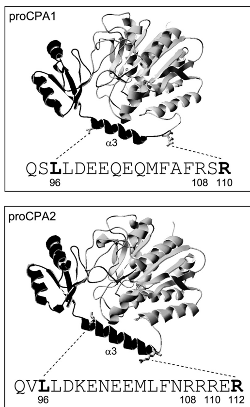
FIGURE 1. Ribbon diagram of porcine proCPA1 (Protein Data Bank code 1PCA) and human proCPA2 (Protein Data Bank code 1AYE). The propeptides are highlighted in black . The amino acid sequences of the \alpha 3 helices and the flanking tryptic activation sites in human proCPA1 and proCPA2 are indicated. The side chains for Leu 96 (proCPA1 and proCPA2), Arg 110 (proCPA1), and Arg 112 (proCPA2) are shown. For clarity, the N-terminal amino acid residues have been removed, and the structures start with Gln 24 . The image was rendered using DeepView/Swiss-PdbViewer (version 3.7).
