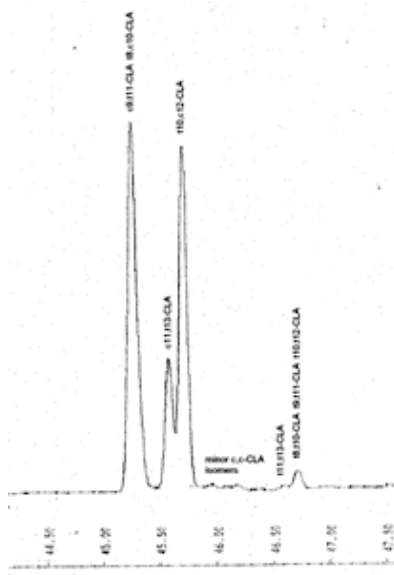
Figure 1: The partial separation of conjugated linoleic acid methyl esters with GC. Standard: ‘Conjugated linoleic acids’ from Sigma. Chrompack CP 9000 GC; 6 \mu L manual split (16:1) injection (270 °C); column: 100 m \times 0.25 mm CP-Sil 88 (FAME) from 130 °C to 225 °C at a rate of 2 °C min -1 , at 225 °C isotherm for 20 min; carrier gas: He (230 kPa, 16.1 cm/s); FID (270 °C)
