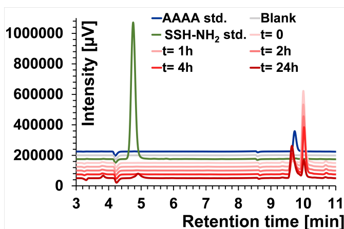
Figure 8. Series of time dependence HPLC chromatograms of the Ni(II): AAAASSH-NH 2 2:1 ratio system at pH = 8.23.
