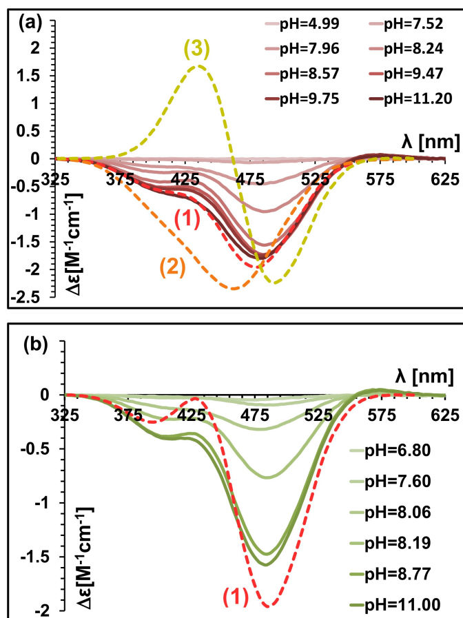
Figure 7. Series of CD spectra depending on pH of the equimolar system, CD spectra of [\text{NiH}_3\text{L}]^- species of AAAA (2), Ac-KGGYTMHK-NH 2 [27] (3) and the model curve of [\text{NiH}_3\text{L}]^- of \text{A}_4\text{SSH-NH}_2 peptide, calculated by summing the CD curves of AAAA and Ac-KGGYTMHK-NH 2 (1) at a ratio of 70%:30% (a); series of CD spectra depending on pH at double nickel(II) ion excess and the model curve of the [\text{Ni}_2\text{H}_6\text{L}]^{2-} of \text{A}_4\text{SSH-NH}_2 peptide (1) calculated by summing the CD curves of AAAA and Ac-KGGYTMHK-NH 2 at a ratio of 50%:50% (b).
