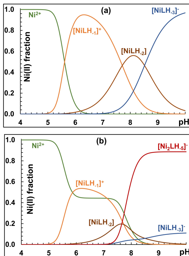
Figure 10. Distribution curves of the systems Ni(II):AAAEKSH-NH 2 = 1:1 (a) and 2:1 (b).
