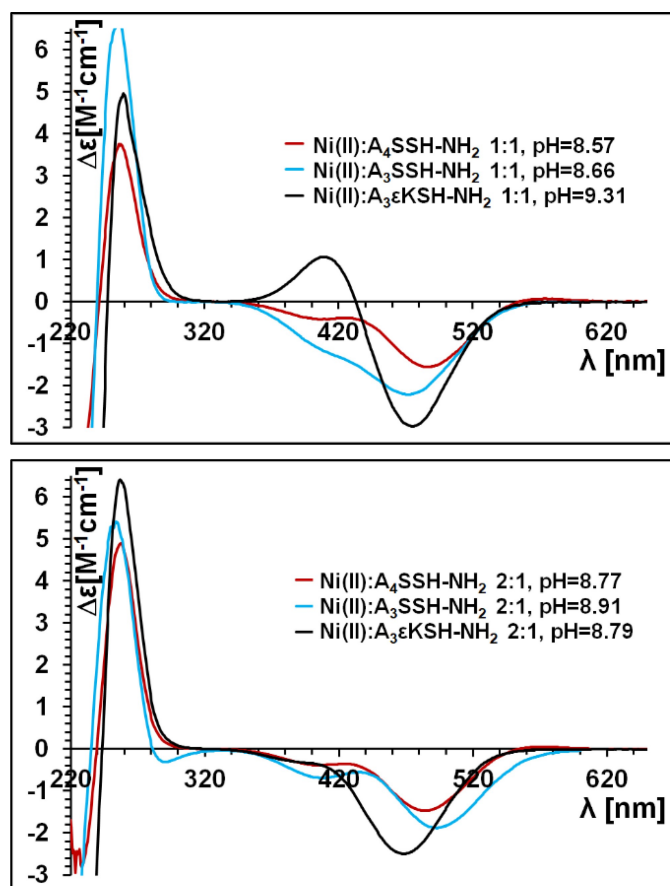
Figure 11. Comparison of the CD spectra of metal complexes formed at alkaline pH in the Ni(II)-ligand 1:1 (a) and 2:1 ratio (b).
