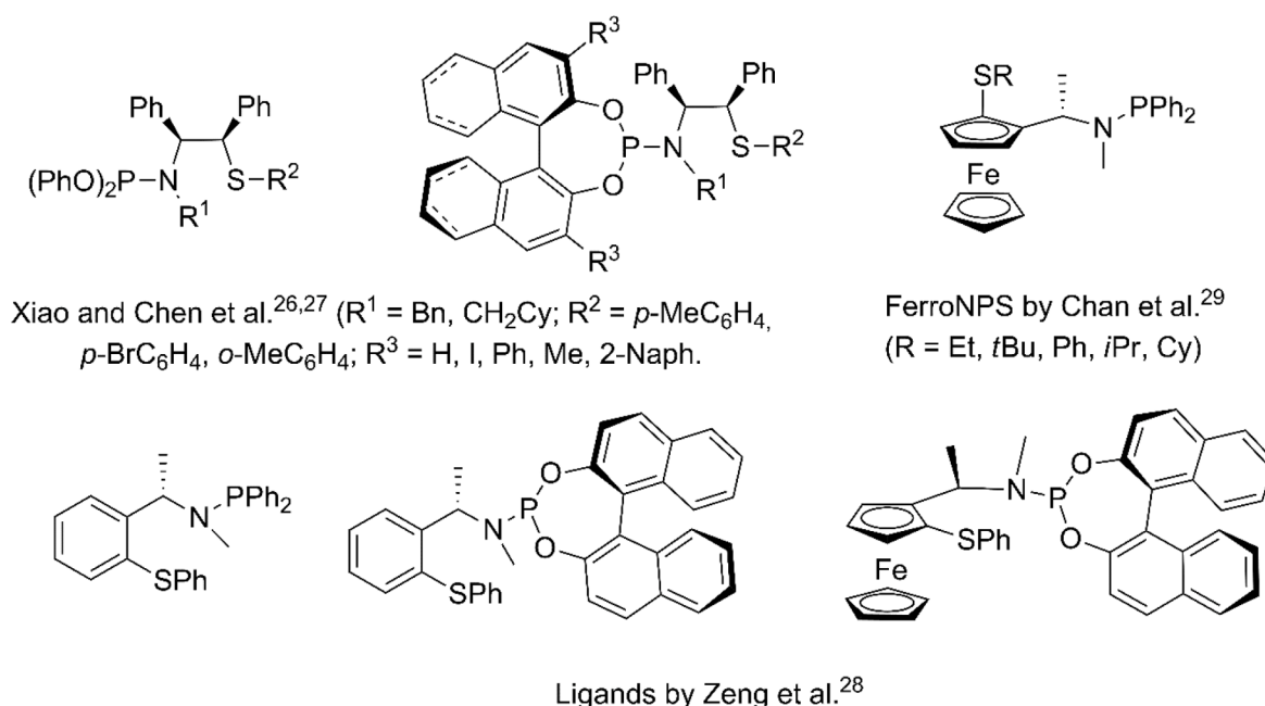
Fig. 1. Thioether-phosphoramidite and thioether-aminophosphine (PN,S) ligands used in asymmetric catalytic transformations.
