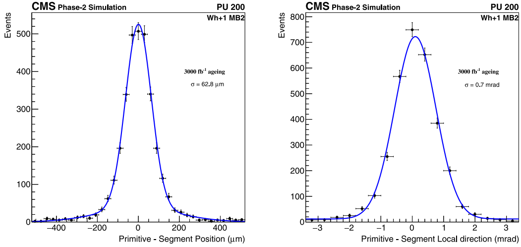
Fig. 4. Difference with respect to offline reconstructed segments of TP local position x_0 (left) and TP local slope \tan \psi (right), for correlated TPs in Wh + 1 MB2. End of HL-LHC ageing is applied to hits before TP generation.
