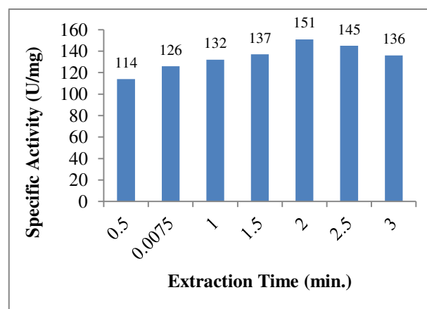
Figure 3: Effect of extraction time on Actinidin extraction from kiwifruit.
