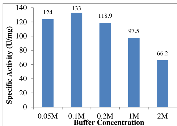
Figure 2 Effect of buffer concentration on Actinidin extraction from kiwifruit.
