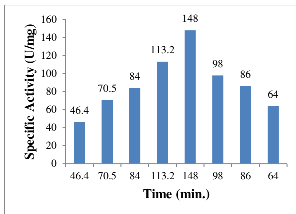
Figure 6: Effect of incubation period on Actinidin activity.
