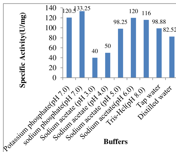
Figure 1: Effect of buffer and pH on Actinidin extraction from kiwifruit.
