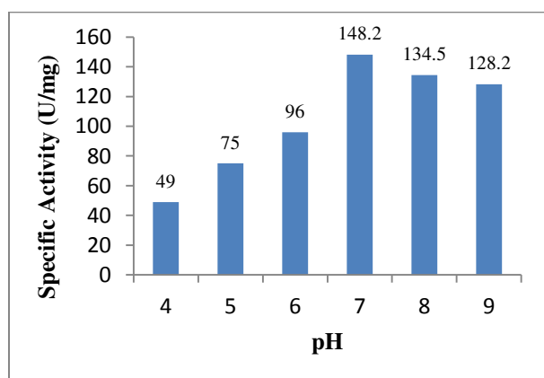
Figure 5: Effect of substrate pH on Actinidin activity.
