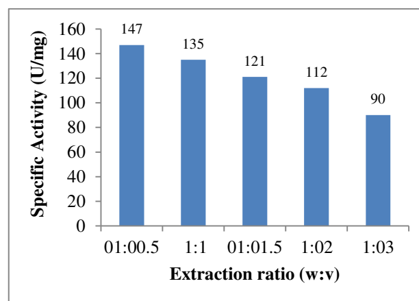
Figure 4: Effect of extraction ratio on Actinidin extraction from kiwifruit.
