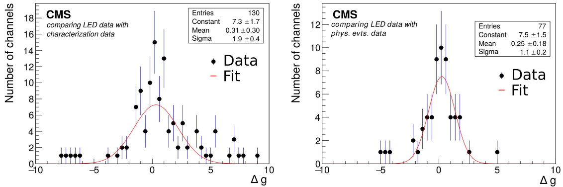
Figure 15. Distributions of the weighed difference of gains, \Delta g = (g_1 - g_2)/\sqrt{\sigma_{g_1}^2 + \sigma_{g_2}^2} , for two sets of correction factors obtained with two different methods, fitted to a Gaussian function. The uncertainties are statistical only. Left: comparison of LED and PMT characterization methods at B = 0 T for muon halo and proton physics HV settings in 2016. Right: comparison of LED and physics events methods for muon halo and heavy ion physics HV settings at B = 3.8 T. Note that in both distributions the number of entries differs from 224 since only a subset of all channels has valid data available in both measurements. The boxes show the parameters of the red Gaussian fit.
