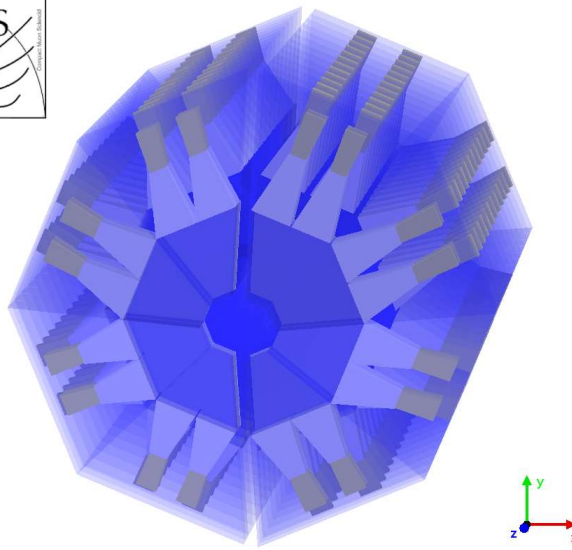
Figure 26. Visualization of the CASTOR detector geometry in simulations. The inner trapezoids in darker blue are the active volumes, while the outer volumes describe the light guides and the PMTs. The near and far halves are placed at the measured position corresponding to the data taking in 2013. An opening of 2.2 cm along the x -axis is visible between the two halves.
