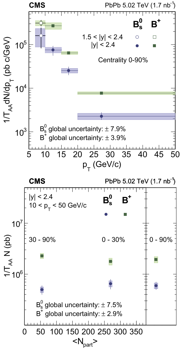
Fig. 2. The acceptance- and efficiency-corrected yields for the B^+ and B^0 mesons, scaled by T_{AA} and N_{MB} in PbPb collisions at \sqrt{s_{NN}} = 5.02 TeV. The results are shown as a function of the meson p_T (upper), and of the event centrality (lower), where the rightmost panel indicates the centrality-integrated result. The vertical bars (boxes) correspond to statistical (systematic) uncertainties. The global systematic uncertainty comprises the uncertainties in T_{AA} , N_{MB} , \mathcal{B} (upper) and \mathcal{B} (lower).
