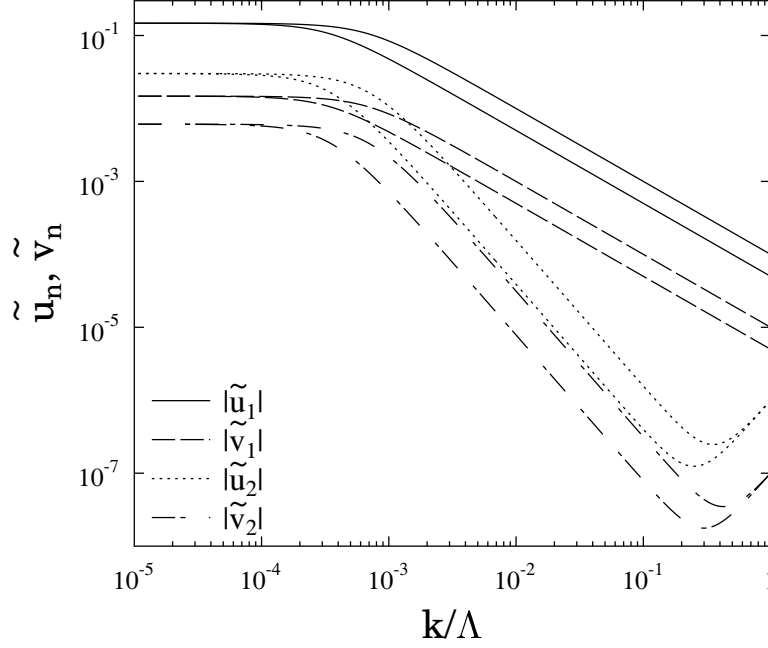
Figure 3. In this figure we show that the IR effective potential of the non-compact MFSG model for \beta^2 = 4\pi depends on only the ratio of the Fourier amplitudes of the fundamental cosine and sine modes. If the P-RG equation has been solved with various initial conditions for \tilde{u}_1(\Lambda) and \tilde{v}_1(\Lambda) but keeping their ratio fixed, then one obtains the same deep IR behavior.
