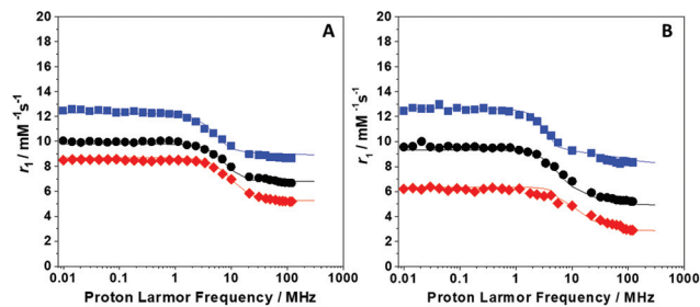
Fig. 2 ^1\text{H} nuclear magnetic relaxation dispersion (NMRD) profiles at pH 7.0 of Gd(AAZ3A-endoHB) (A) and Gd(AAZ3A-exoHB) (B) recorded at different temperatures 283 K (■), 298 K (●) and 310 K (◆). The solid lines correspond to the fits of the data as described in the text.
