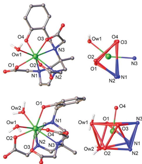
Fig. 1 Structures of the [Gd(AAZ3A-endoHB)(H 2 O) 2 ] - (bottom) and [Gd(AAZ3A-exoHB)(H 2 O) 2 ] - (top) systems obtained with DFT calculations. Second-sphere water molecules are omitted for simplicity. Bond distances (Å), [Gd(AAZ3A-endoHB)(H 2 O) 2 ] - : Gd–N1, 2.734; Gd–N2, 2.725; Gd–N3, 2.701; Gd–O1, 2.391; Gd–O2, 2.426; Gd–O3, 2.402; Gd–O4, 2.452; Gd–O1w, 2.515; Gd–O2w, 2.518. [Gd(AAZ3A-exoHB)(H 2 O) 2 ] - : Gd–N1, 2.661; Gd–N2, 2.649; Gd–N3, 2.681; Gd–O1, 2.403; Gd–O2, 2.421; Gd–O3, 2.360; Gd–O4, 2.325; Gd–O1w, 2.470.
