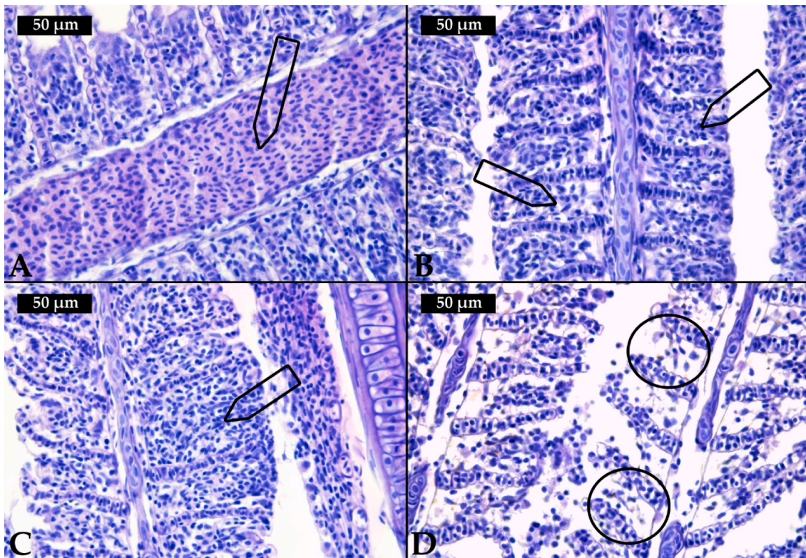
Fig. 1. Histological alterations in the carp gills after cypermethrin (CYP) exposure (H&E): A – vasodilation of central sinus at 0.0002 µg/L; B – fusions of the secondary lamellae at 0.0003 µg/L; C – epithelial proliferation at 0.0006 µg/L; D – necrosis at 0.0006 µg/L.
