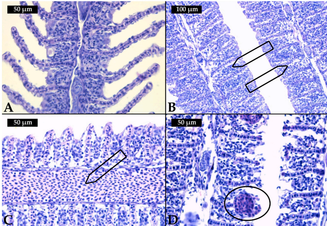
Fig. 2. Histological alterations in the carp gills after chlorpyrifos (CPF) exposure (H&E): A – control gills; B – fusion of the secondary lamellae at 0.03 µg/L; C – vasodilation of central sinus at 0.05 µg/L; D – aneurysms in the secondary lamellae at 0.1 µg/L.
