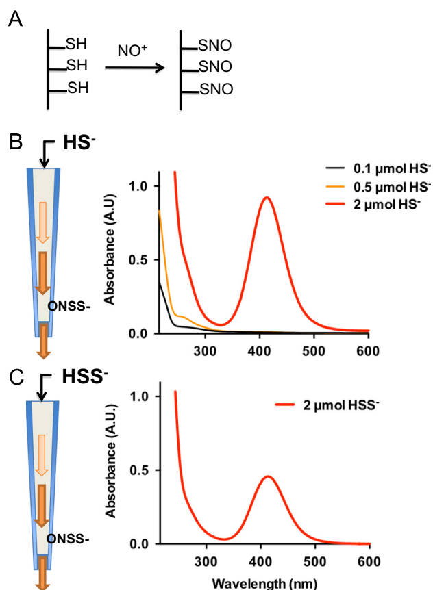
Fig. 5. Formation of \text{SSNO}^- from the reaction between sulfide and immobilized S-nitroso moieties. (A) S-nitrosation by acidified nitrite of resin-bound sulfhydryl (–SH) groups (Ekathiol®) to form an immobilized nitrosothiol. (B,C) A solution of either \text{Na}_2\text{S} (B) or \text{Na}_2\text{S}_2 (C) is passed over the column and reacts with immobilized S-nitrosothiols to form \text{SSNO}^- ( \lambda_{\text{max}} 412 nm; high sulfide concentration) and polysulfides (< 280 nm; lower sulfide concentrations). Depicted results are representative of 4 independent experiments with different batches of nitrosated thiol-containing resin and various absolute amounts of sulfide (0.015–5 \mu\text{moles} on column).
