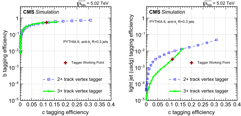
Fig. 1. Efficiency of tagging b jets (left) and light parton jets (right) for the high-purity (3+ track), and high-efficiency (2+ track) versions of the simple secondary vertex (SSV) tagger as a function of c jet tagging efficiency. The charm-to-bottom discrimination power is virtually unchanged between the high-efficiency and high-purity versions of the tagger, while the light parton jet mistag rate is reduced by a factor of three at the analysis working point, shown as the closed red cross on the plots. (For interpretation of the references to color in this figure, the reader is referred to the web version of this article.)
