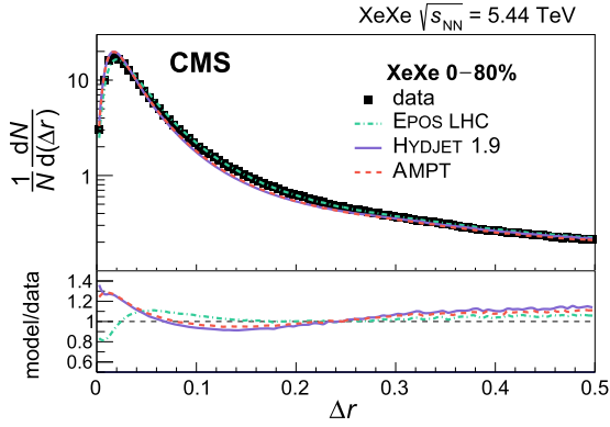
Fig. 1. The \Delta r distributions for tracklets reconstructed from the two layers of the BPX closest to the beam pipe. The distributions are normalised by the number of tracklets. The spectrum in collision data (black squares) is compared to the spectra obtained from fully simulated events generated with Epos LHC v3400 [8,18], HYDJET 1.9 [9], and AMPT 1.26t5 [19]. The ratio of the distributions in simulation to data is shown in the bottom panel. The statistical uncertainties are smaller than the marker sizes for all distributions shown.
