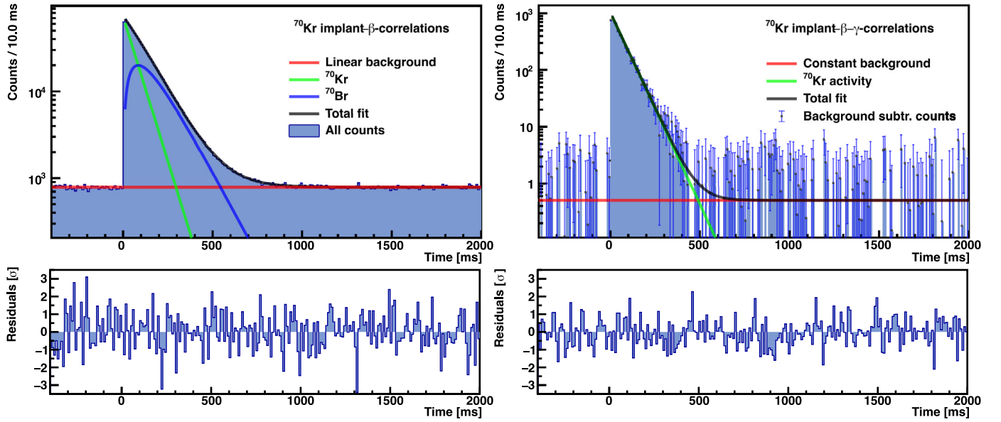
Fig. 1. The time distribution of i\text{-}\beta (left) and i\text{-}\beta\text{-}\gamma (right) correlations. The fitting function for the i\text{-}\beta time distribution includes the Bateman formula for the ^{70}\text{Kr} and ^{70}\text{Br} decays, assuming a value of 78.42 \pm 0.51 ms [38] for the half-life of ^{70}\text{Br} and a background term extracted from a linear fit to the backward-time distribution of i\text{-}\beta correlations. The black, green, blue and red curves correspond to the total fit, the resulting partial activities and to the background, respectively. In the case of the i\text{-}\beta\text{-}\gamma correlations the total fit is the sum of the identified, high-intensity \gamma -peaks' activities which is calculated from the subtraction of the time distribution of the total area of the peaks, the Compton-background activity, and a constant background. The black, green and red curves correspond to the total fit, the sum of the \gamma -peak activities and the background, respectively.
