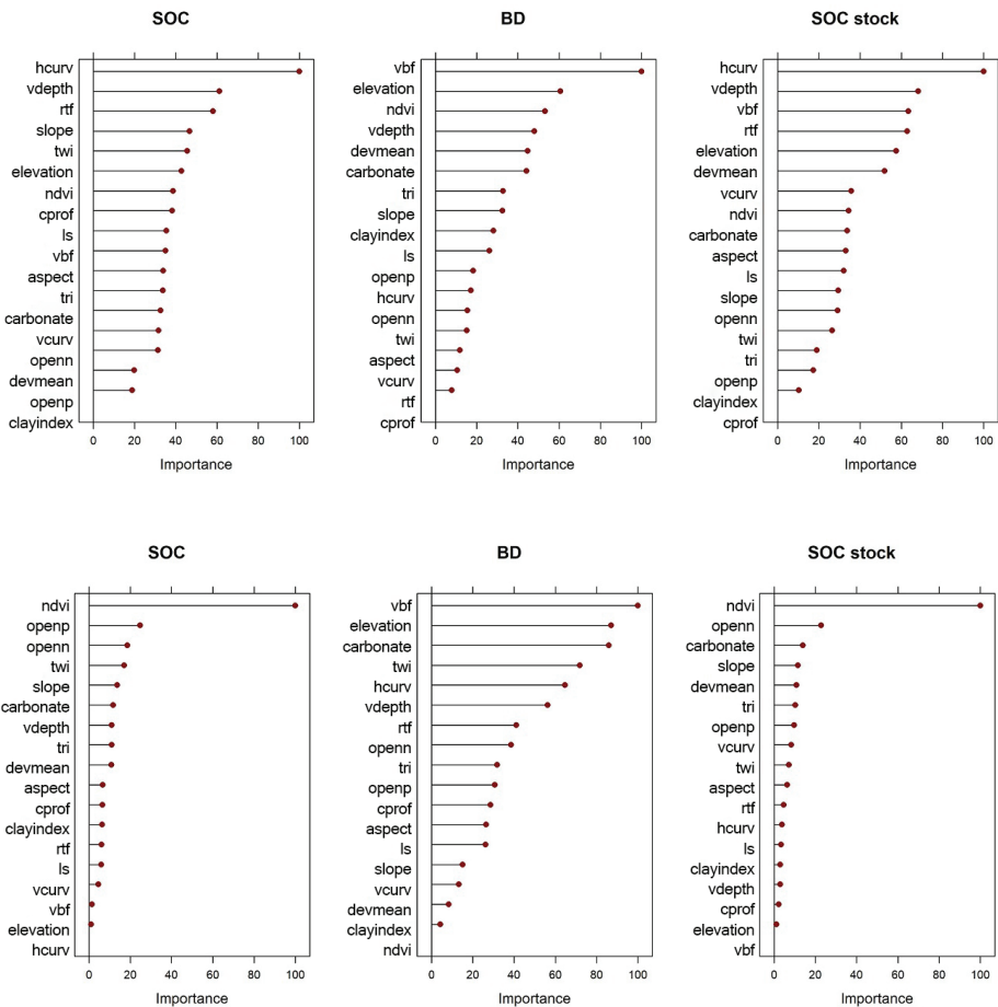
Fig. 7. Variable importance based on RF for each properties in Látókép. Abbreviations: hcurv and vcurve: plan and profile curvature, ls: ls-factor, opennessp and opennessn: positive and negative openness, tri: terrain ruggedness index, vbf: multiresolution index of valley bottom flatness, rtf: multiresolution index of ridge top flatness, twi: topographic wetness index, vdepth: valley depth, devmean: deviation from mean value, carbonate: carbonate normalized ratio, NDVI: normalized difference vegetation index, SOC stock: soil organic carbon stock, and BD: bulk density.
