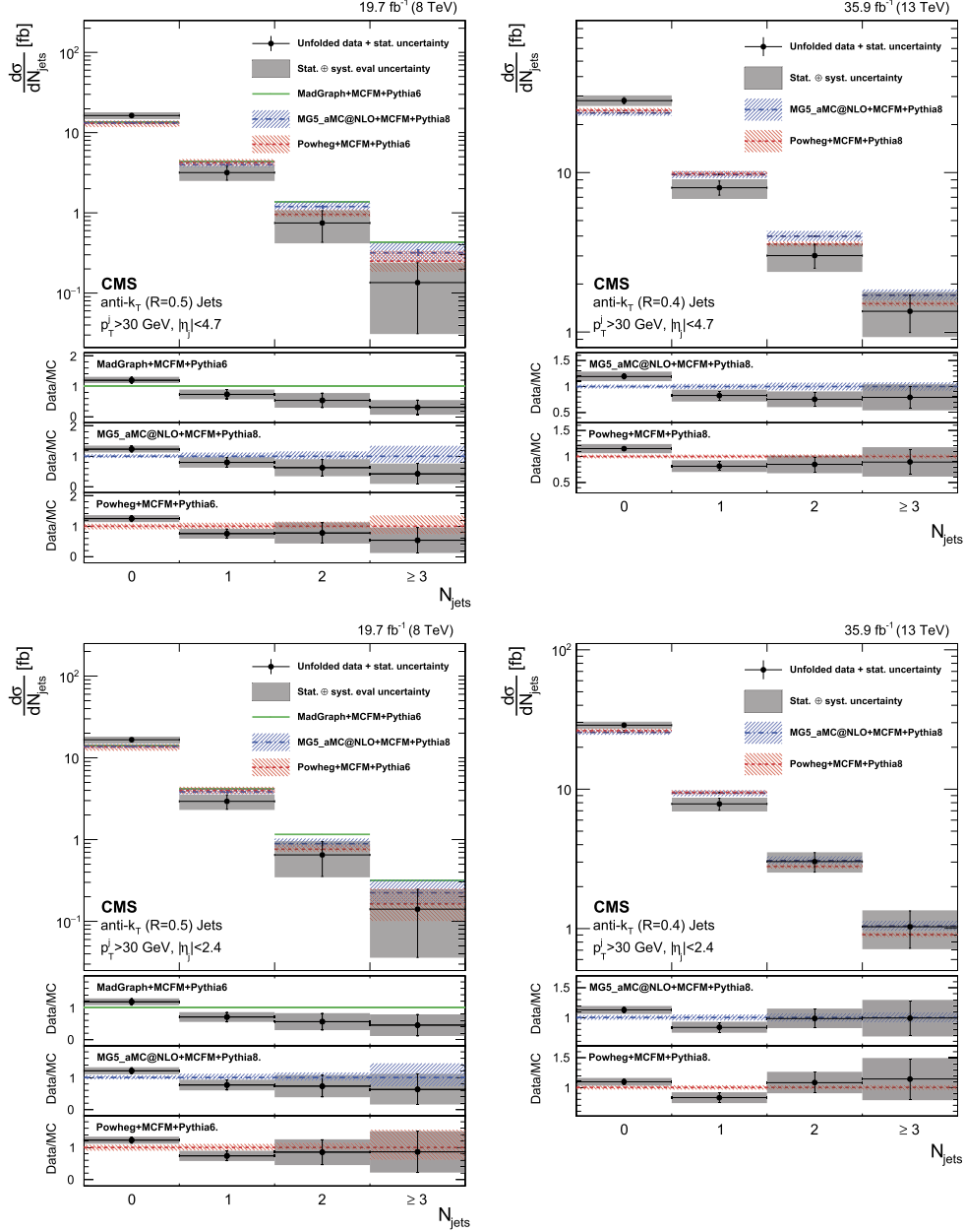
Fig. 2. Differential cross sections of pp \rightarrow ZZ \rightarrow 4\ell as a function of the multiplicity of jets with |\eta_{\perp}| < 4.7 (top panels) and |\eta_{\perp}| < 2.4 (bottom panels), for the 8 (left) and 13 (right) TeV data. The measurements are compared to the predictions of MG5_aMC@NLO, POWHEG, and MADGRAPH5 (8 TeV only) sets of samples. Each MC set, along with the main MC generator, includes the MCFM and PHANTOM generators. PYTHIA 6 and PYTHIA 8 are used for parton showering, hadronization, and underlying event simulation, for the 8 and 13 TeV analysis, respectively, with the sole exception of MG5_aMC@NLO, which is always interfaced to PYTHIA 8. The total experimental uncertainties are shown as hatched regions, while the colored bands display the theoretical uncertainties in the matrix-element calculations.
