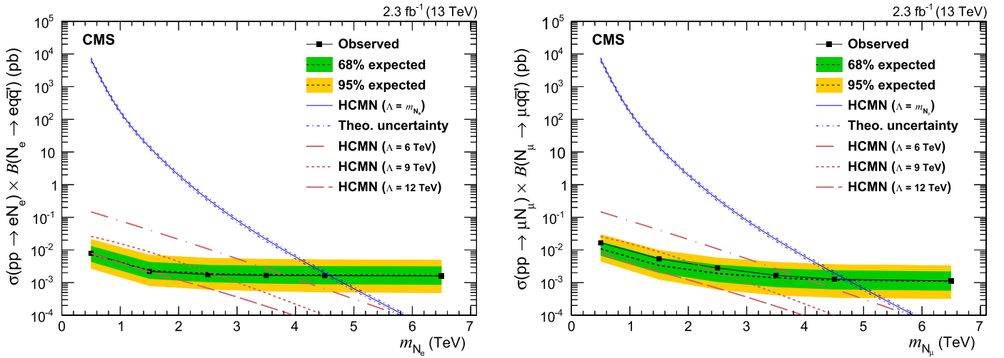
Fig. 5. The observed 95% CL upper limits (solid black lines) on \sigma(pp \rightarrow \ell N_\ell) B(N_\ell \rightarrow \ell q\bar{q}') , obtained in the analysis of the ee\bar{q}\bar{q}' (left) and the \mu\mu q\bar{q}' (right) final states, as a function of the mass of the heavy composite Majorana neutrino, N_\ell . The corresponding expected limits are shown by the dotted lines, and the bands represent the expected variation of the limit to one and two standard deviation(s). The solid blue curve indicates the theoretical prediction of \sigma(pp \rightarrow \ell N_\ell) B(N_\ell \rightarrow \ell q\bar{q}') for \Lambda = m_{N_\ell} . The uncertainty in the theoretical prediction is derived by taking into account the factorization and normalization scales. The light red textured curves give the theoretical predictions for three \Lambda values ranging from 6 to 12 TeV in steps of 3 TeV. (For interpretation of the references to colour in this figure legend, the reader is referred to the web version of this article.)
