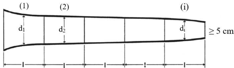
Figure 2: Sectionize measurements on felled trees. Based on Laar and Akça (2007)
