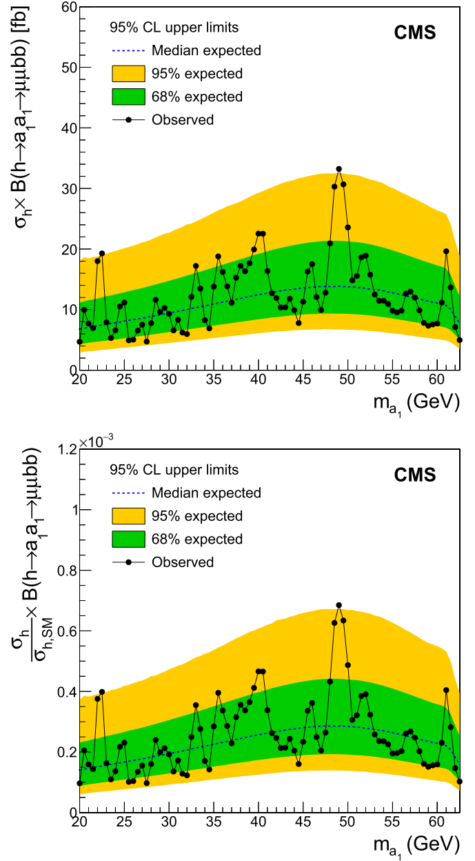
Fig. 5. Observed and expected upper limits at 95% CL on the (upper) product of the Higgs boson production cross section and \mathcal{B}(h \rightarrow a_1 a_1 \rightarrow \mu^+ \mu^- b \bar{b}) and (lower) the branching fraction as a function of m_{a_1} . The inner and outer bands indicate the regions containing the distribution of limits located within 68 and 95% confidence intervals, respectively, of the expectation under the background-only hypothesis.
