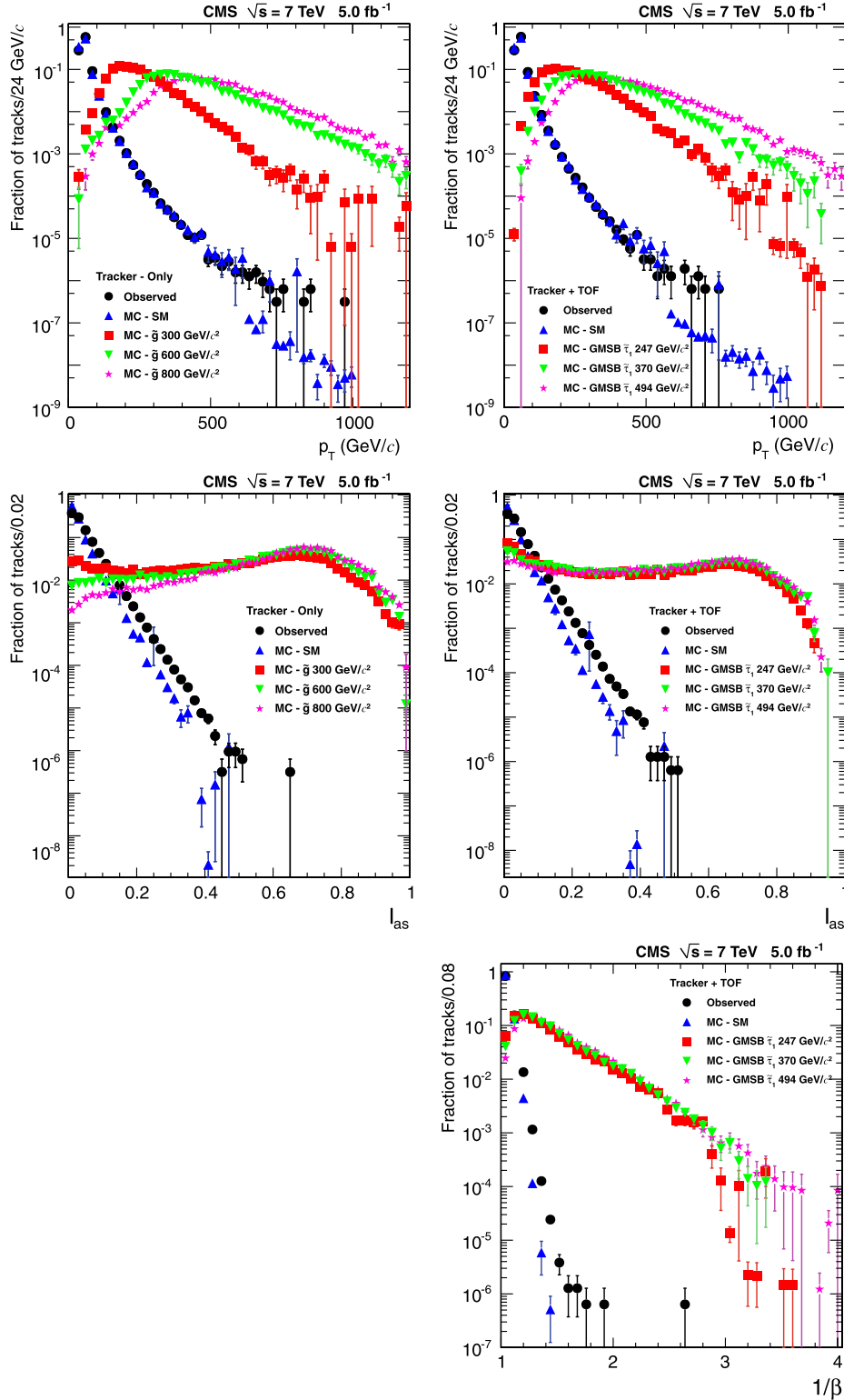
Fig. 1. Normalized distributions of p_T , l_{as} , and \beta^{-1} in data, simulated SM processes, and some of the simulated signal samples. The two plots on the left are for the tracker-only selection. The three plots on the right are for the tracker + TOF selection. Different simulated signal samples are used for the left and right plots.
