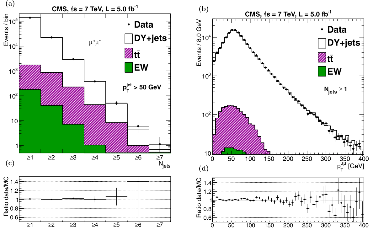
Fig. 2. Distributions for Z \rightarrow \mu\mu candidate events in data, compared with expectations from simulated signal and background contributions using MADGRAPH simulations normalized to the integrated luminosity of the data: (a) as a function of associated jet multiplicity N_{\text{jets}} , and (b) as a function of p_T of the dimuon pair ( p_T^{\mu\mu} ) for N_{\text{jets}} \geq 1 . The dibosons WW, WZ, ZZ and W + jets backgrounds are collectively denoted as EW in the legends. The plots in (c) and (d) show the ratios of the data to predictions from MC. The error bars on the data points represent only their statistical uncertainties and do not include systematic effects.
