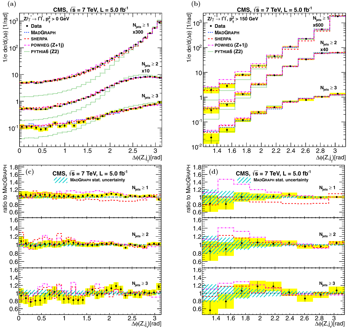
Fig. 4. Normalized \Delta\phi(Z, j_1) distributions for the leading jet in the inclusive jet multiplicity bins N_{\text{jets}} \geq 1, \geq 2 , and \geq 3 : (a) all p_T^Z and (b) p_T^Z > 150 GeV. Plots in (c) and (d) show the corresponding ratios of the data (solid points), and of other MC predictions, relative to MADGRAPH. The ratio for PYTHIA MC is not included in these plots. The error bars on the data points represent their statistical uncertainties, the solid yellow shaded band around the points represents the sum of statistical and systematic uncertainties taken in quadrature, while the cross-hatched (cyan) bands reflect the statistical uncertainties on the MADGRAPH calculations. (For interpretation of the references to color in this figure legend, the reader is referred to the web version of this Letter.)
