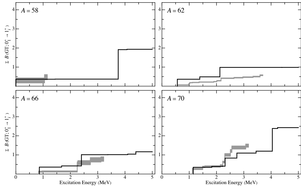
Figure 6. Distributions of the GT strength in the decay from N = Z - 2 to N = Z nuclei for A = 58, 62, 66, and 70 . The experimental B(\text{GT}) distributions and their uncertainties are indicated in grey. Parameters of the Hamiltonian (31) are given in Table 3 and the GT strength is calculated with a quenching factor q^2 = 0.74^2 .
