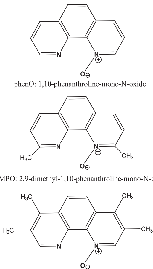
Scheme 1. The phenanthroline-mono- N -oxides used in this study.
