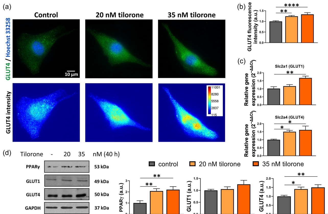
FIGURE 3 Tilorone increases the expression of glucose transporters (GLUTs). (a) Representative wide-field fluorescence images reveal the distribution of GLUT4 following staining with Alexa Fluor 488 (green). Nuclei were stained by Hoechst 33258 (blue). Representative pseudocolor images depict the GLUT4 signal intensity. The color was assigned to each pixel based on the pixel intensity value according to the calibration bar. (b) The mean intensity values of the cells were quantified, normalized to control, and compared following tilorone treatment. Data are reported as the mean + SEM ( n = 3 independent experiments, 36–41 cells/treatment were quantified). (c) The levels of Slc2a1 (GLUT1) and Slc2a4 (GLUT4) were studied by quantitative real-time PCR. The housekeeping genes MmHprt and MmRpl27 were used as internal controls to normalize qRT-PCR results, and relative gene expression levels were calculated using the 2^{-\Delta\Delta Ct} method. Data are reported as the mean + SEM ( n = 3 –4 independent experiments). (d) Representative western blots of PPAR \gamma , GLUT1, and GLUT4 protein expression. GAPDH was used as an internal control. Quantification of the results normalized to control and reported as the mean + SEM (GLUT1: n = 3 , PPAR \gamma and GLUT4: n = 8 independent experiments). * p < 0.05 , ** p < 0.01 , *** p < 0.0001 . au, arbitrary unit; PPAR \gamma , peroxisome proliferator-activated receptor- \gamma .
