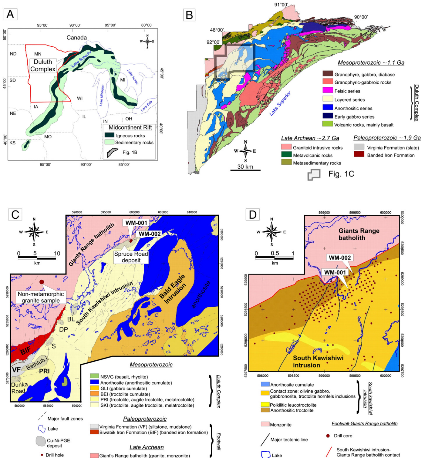
Fig. 1. (A) The Midcontinent Rift system in North-America (modified after Ojakangas et al., 2001). (B) Geologic map of the DC. The South Kawishiwi intrusion, studied in this work is highlighted by a black square. (C) Geology of the SKI and its surroundings. Abbreviations: BL – Birch Lake Deposit, DP – Dunka Pit Deposit, S – Serpentine Deposit, Partridge River intrusion. (D) Detailed geologic map of the Spruce Road deposit.
