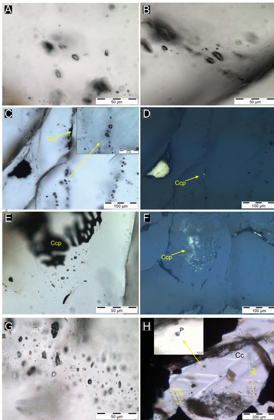
Fig. 9. (A) Cluster of Type I, early \text{CO}_2 fluid inclusions in the recrystallized quartz porphyroblast. (B) Three-phase (Laq, Lcar, Vcar) Type II, secondary \text{CO}_2 - \text{H}_2\text{O} -NaCl fluid inclusions in the recrystallized quartz porphyroblast. (C) Three-phase Type II, secondary \text{CO}_2 - \text{H}_2\text{O} -NaCl fluid inclusions in the recrystallized quartz porphyroblast. Note the chalcopyrite inclusions along the fluid inclusion planes. (D) Same area as panel C under reflected light. (E) Type III \text{CH}_4 - \text{N}_2 - \text{H}_2\text{O} secondary fluid inclusions associated to chalcopyrite inclusions in fluid inclusion planes. (F) Same area as panel E under reflected light. (G) Pure \text{CH}_4 - \text{N}_2 and \text{H}_2\text{O} -NaCl inclusions along the same fluid inclusion trail. (H) Primary and secondary Type IV \text{CaCl}_2 -NaCl- \text{H}_2\text{O} fluid inclusions in calcite II.
