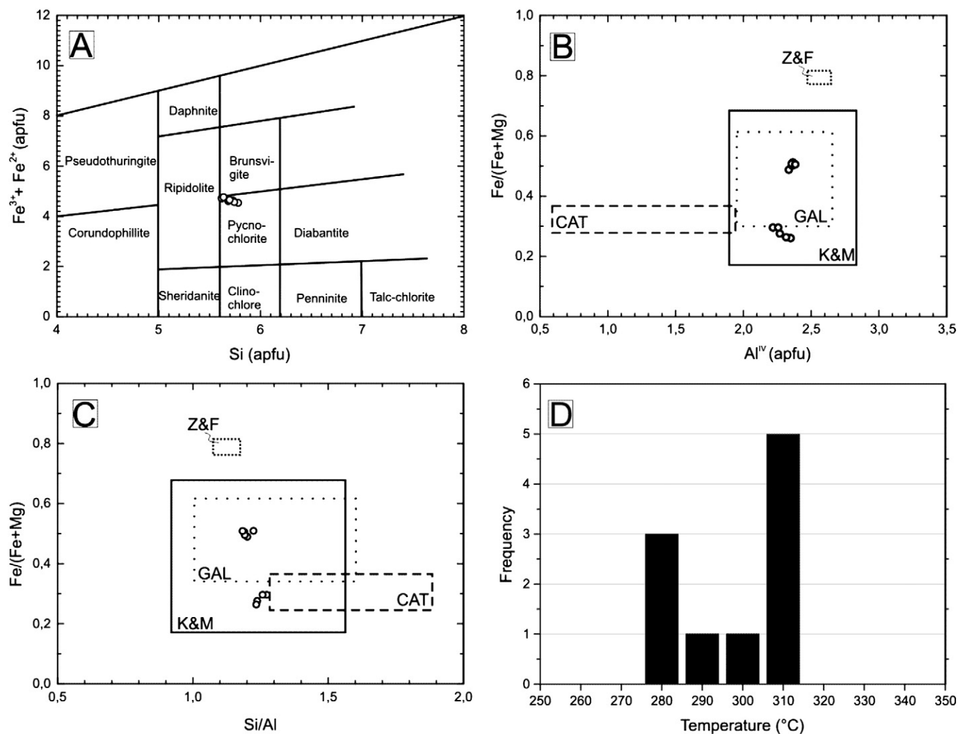
Fig. 7. (A) Classification of chlorites based on the diagram of Hey (1954). (B–C) Comparison of chlorite compositions from the charnockitic footwall of the SKI with those used for empirical temperature estimation of Cathelineau (1988), Kranidiotis and MacLean (1987), and Zang and Fyfe (1995). Compositional fields of the Anorthositic series of the SKI of the DC (Gál et al., 2011) are plotted for reference. (D) Histogram of crystallization temperatures of chlorites calculated by the empirical method of Kranidiotis and MacLean (1987).
