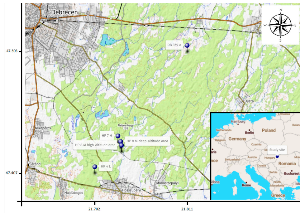
Figure 3. Sampling locations in the Southern Nyírség (Hungary)
