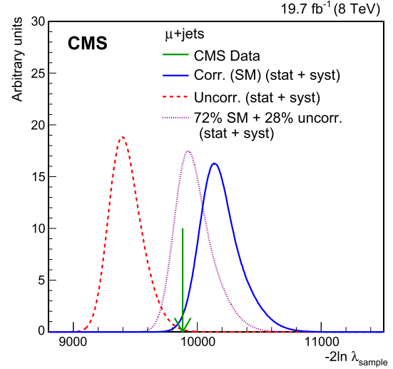
Fig. 6. The -2\ln\lambda_{\text{sample}} distribution in simulation, evaluated for the data set size. The samples in simulation contain signal and background mixed according to the theoretical cross sections, with the solid distribution obtained using SM t\bar{t} simulation and the dashed distribution obtained using uncorrelated t\bar{t} simulation, including systematic uncertainties. The arrow indicates the -2\ln\lambda_{\text{sample}} observed in data. The dotted curve shows a mixture of 72% SM t\bar{t} events and 28% uncorrelated t\bar{t} events.
