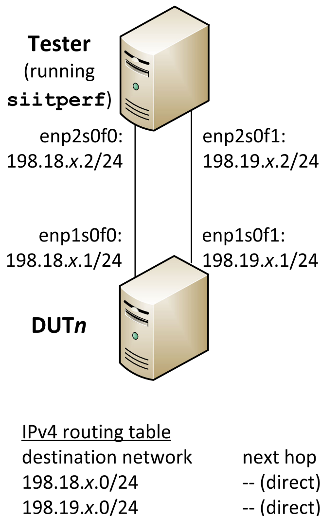
FIGURE 4 Single DUT test setup for IPv4 packet forwarding rate measurements.
