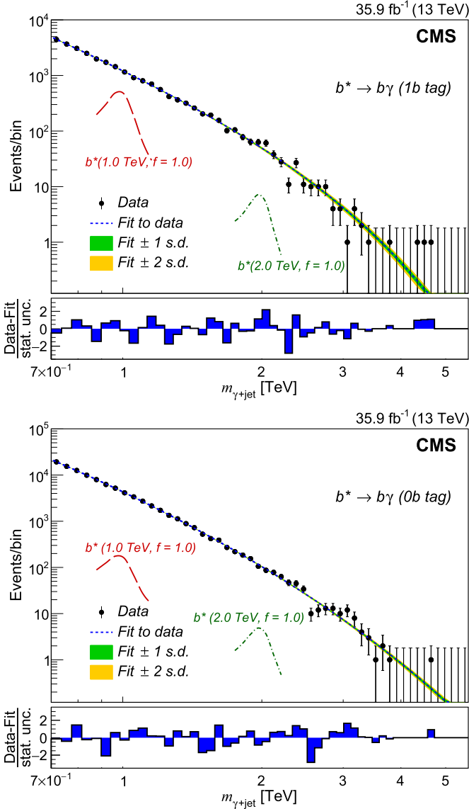
Fig. 3. The \gamma + b_{\text{jet}} invariant mass distribution in data (black points) used for the b^* analysis, after final selection for (upper) 1b tag category and (lower) 0b tag category. The result of the fit to the data using the parametrization defined in Eq. (2) is shown by the blue dashed curve with associated bands indicating the uncertainty. The bin-by-bin pull, (\text{Data-Fit})/(\text{stat. unc.}) , where the denominator refers to the statistical uncertainty in data, is also presented. The green and yellow bands correspond to 1 and 2 standard deviations, respectively from the mean value. Simulations of excited b quark signals representing the expected excess of signal events over the background are shown for the 1b and 0b tag categories for the mass values of 1.0 and 2.0 TeV for f = 1.0 .
