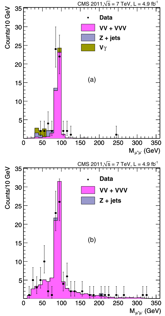
Fig. 2. Distributions of the \mu^-\mu^+ invariant mass for (a) \mu^-e^+\mu^+ and (b) \mu^-e^+\mu^+ events in data (black points), before applying any requirement on the \mu^-\mu^+ mass to reject Z bosons, compared to the sum of all major SM background contributions.
