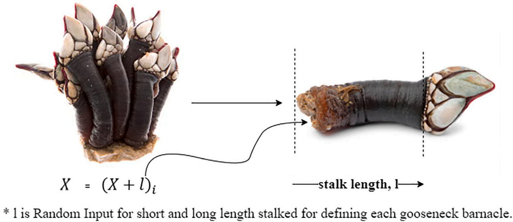
Fig. 5. Hardy-Weinberg principles.
