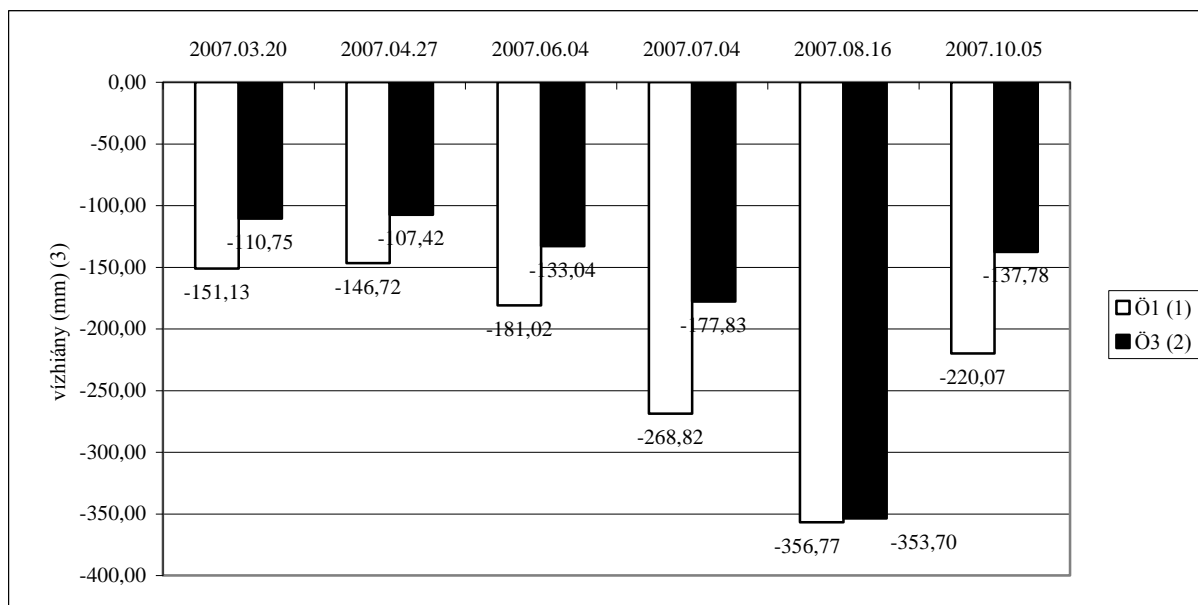
Figure 2: Dynamic changing of water deficit of maize in biculture (Debrecen, chernozem soil, 2007), (1) not irrigated, (2) irrigated, (3) water deficit
