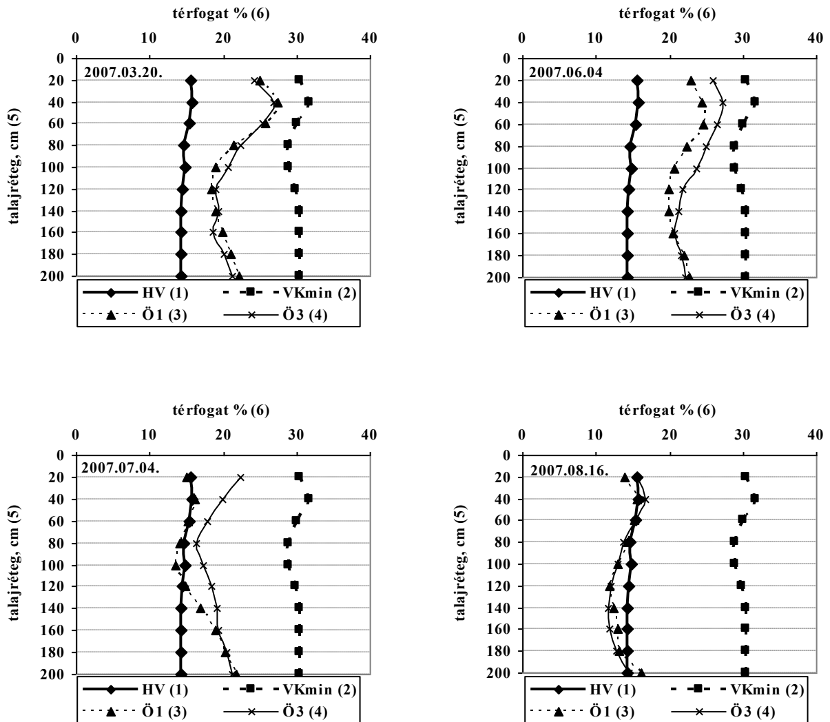
Figure 8.: Changes of watersupply of soil in not irrigated and irrigated treatments in triculture, (1) deadwatercontent, (2) minimal watercapacity, (3) not irrigated treatment, (4) irrigated treatment, (5) stratum, (6) volume
