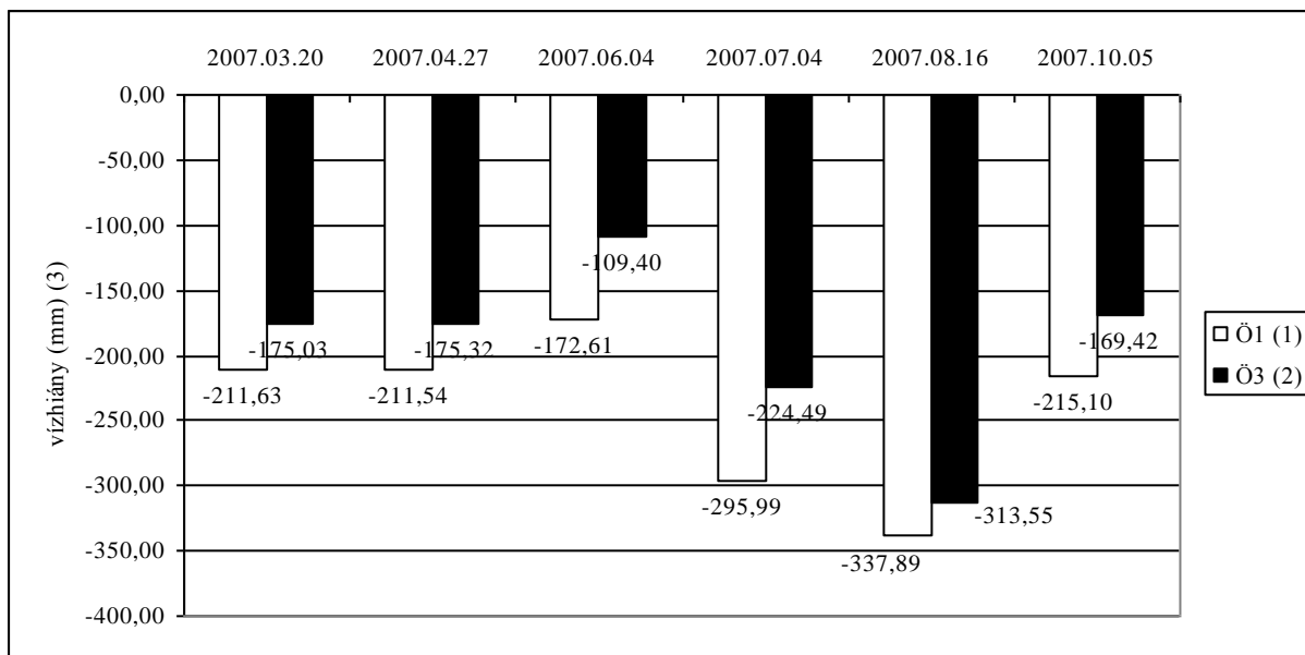
Figure 1: Dynamic changing of water deficit of maize in monoculture (Debrecen, chernozem soil, 2007), (1) not irrigated, (2) irrigated, (3) water deficit
