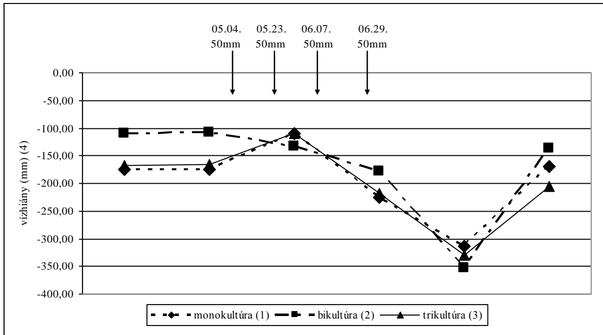
Figure 5.: Effect of precipitation and irrigation on waterdeficit dynamics of irrigated soil in mono-, bi- and triculture (Debrecen, 2007), (1) monoculture, (2) biculture, (3) triculture, (4) water deficit
