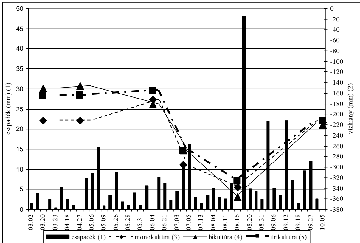
Figure 4.: Precipitation data of crop year of 2007. and water deficit data of not irrigated treatment in mono-, bi- and triculture, (1) precipitation, (2) water deficit, (3) monoculture, (4) biculture, (5) triculture
