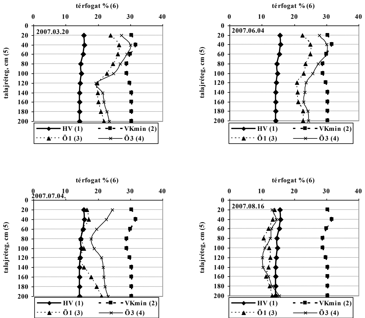
Figure 7.: Changes of watersupply of soil in not irrigated and irrigated treatments in biculture, (1) deadwatercontent, (2) minimal watercapacity, (3) not irrigated treatment, (4) irrigated treatment, (5) stratum, (6) volume %
