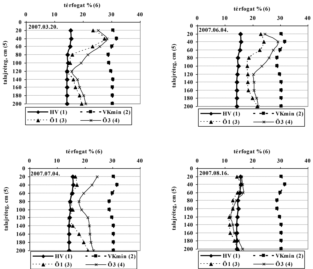
Figure 6.: Changes of watersupply of soil in not irrigated and irrigated treatments in monoculture, (1) deadwatercontent, (2) minimal watercapacity, (3) not irrigated treatment, (4) irrigated treatment, (5) stratum, (6) volume %
