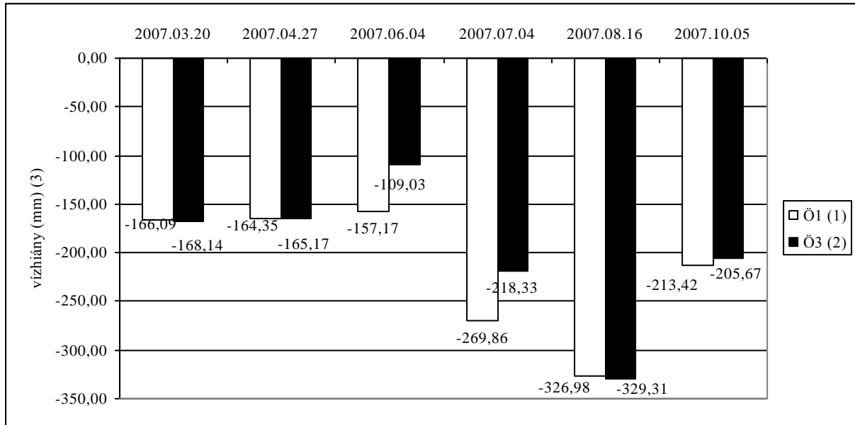
Figure 3: Dynamic changing of water deficit of maize in triculture (Debrecen, chernozem soil, 2007), (1) not irrigated, (2) irrigated, (3) water deficit
