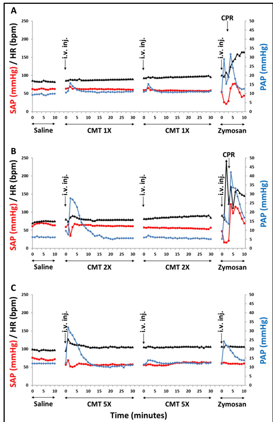
Fig. 1 Time courses of mean systemic (SAP) and pulmonary (PAP) arterial blood pressure and heart rate (HR) changes following 2 consecutive i.v. injections of pigs with 1x (Panel A), 2x (B), and 5x (C) human vaccine dose of Comirnaty. The timing of injections and length of observations are shown by arrows. The y-axis gives the units, separately for SAP and HR (left y-axis) and PAP (right y-axis). Panels A and B show animals pretreated with zymosan 46 and 49 days earlier (pig no. 1 and 2, respectively). Panel C was a naïve pig (no. 10). All animals were injected with 0.1 mg/kg zymosan at the end of the experiments. The HVD expressed as mg/kg for each vaccine component is specified in Table 2. Abbreviations: i.v. inj. , intravenous injection
