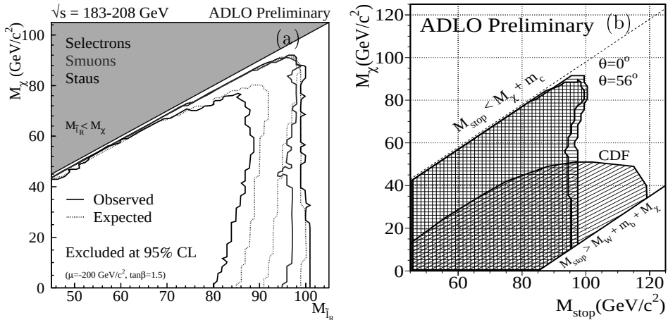
Fig. 1. (a) 95% C.L. exclusion domain in the plane (M_{\tilde{l}}, M_\chi) for the right selectron, the right smuon and the stau in the vanishing coupling to Z condition, using all data collected by the 4 LEP experiments at centre-of-mass energies between 183 and 208 GeV [5]. The observed and the expected limits are given by the full and the dotted lines respectively. The gray region is not kinematically allowed; (b) Excluded region at 95% C.L. in the plane (M_{\tilde{t}}, M_\chi) for two values of mixing angle corresponding to the minimal ( \theta = 56^\circ ) and the maximal ( \theta = 0^\circ ) coupling to Z [6]. The region denoted CDF is excluded by the CDF Collaboration [7].
