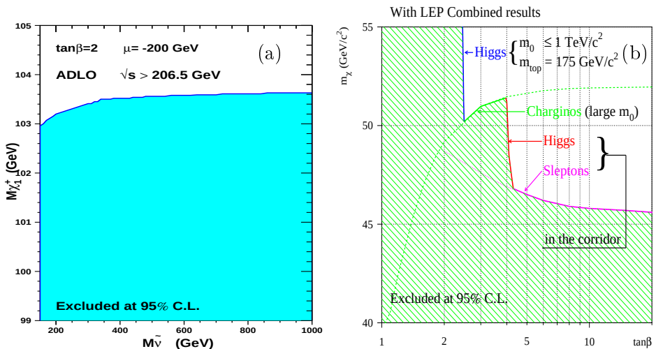
Fig. 2. (a) 95% C.L. exclusion domain in the plane ( M_{\chi_1^+} , M_{\tilde{\nu}} ) at centre-of-mass energies up to 208 GeV ( \tan\beta = 2 and \mu = -200 \text{ GeV}/c^2 ) [8]; (b) Lower limit at 95% C.L. on the neutralino LSP mass as a function of \tan\beta obtained combining the results from the charginos, sleptons and Higgs searches at centre-of-mass energies up to 208 GeV [12]. The lines are used to distinguish the contributions of each analysis.
