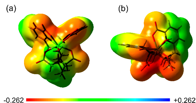
Figure 6. Electrostatic potential (a. u.) mapped on isoelectronic surfaces of 0.001 a. u. for [Y(CHXOITAPA)(H_2O)]^- (a) and [Y(CHXOCTAPA)(H_2O)]^- (b).
