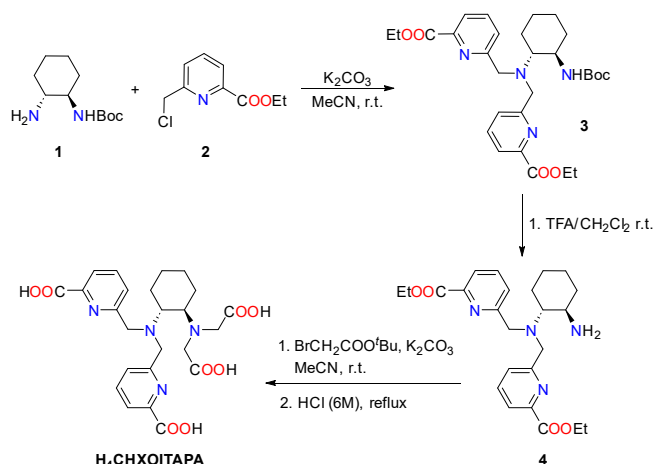
Scheme 1. Synthesis of H 4 OITAPA.
