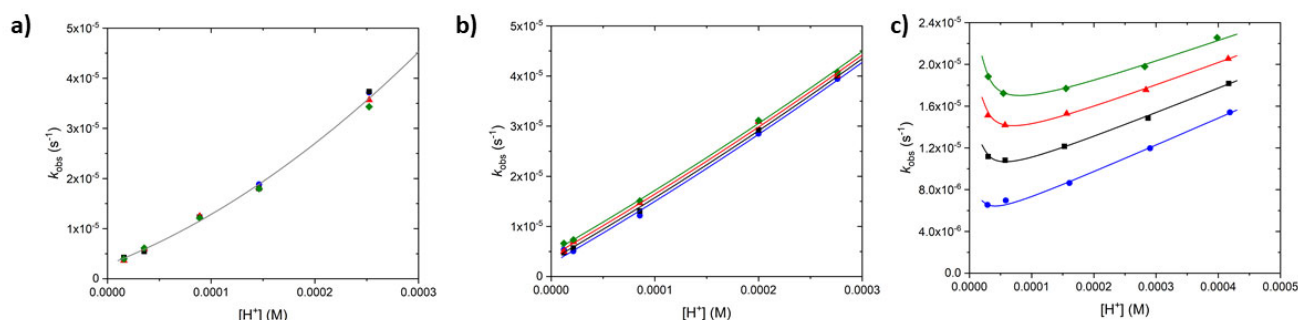
Figure 5. Plot of the pseudo-first-order rate constants measured for the dissociation of the complexes as a function of H + ion concentration (50 mM DMP, 25 °C, 0.15 M NaCl) using different metal ion excess; a) [Lu(CHXOITAPA)] - [10× (3.02 mM), 20× (6.04 mM), 30× (9.06 mM), and 40× (12.08 mM) at pH = 3.66, 3.89, 4.05, 4.43, and 4.76]; b) [Y(CHXOITAPA)] - [10× (3.95 mM), 20× (7.90 mM), 30× (11.8 mM), and 40× (17.78 mM) at pH = 3.56, 3.70, 4.07, 4.67, and 4.91]; c) [Y(CHXOCTAPA)] - [10× (5.53 mM), 20× (11.07 mM), 30× (16.60 mM), and 40× (22.14 mM) at pH = 3.30, 3.50, 3.80, 4.17, and 4.49].
