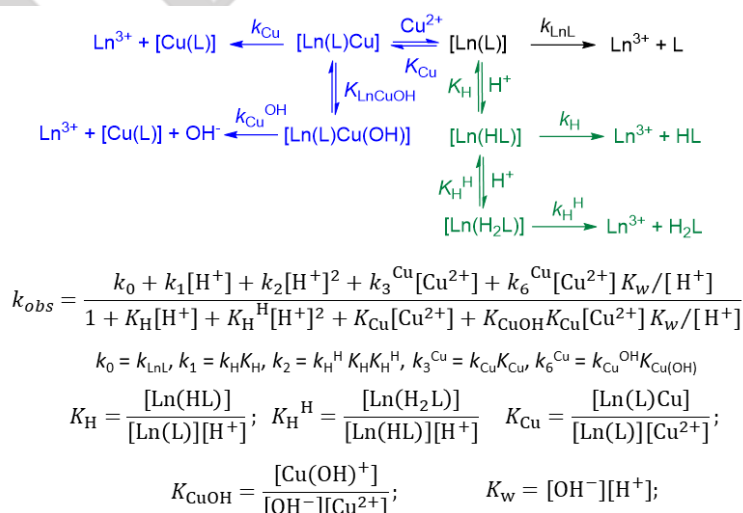
Scheme 2. Dissociation pathways of the Y 3+ and Lu 3+ complexes investigated in this work: spontaneous (black), proton-assisted (green) and metal-assisted (blue) and expressions used to analyze the kinetic data.
