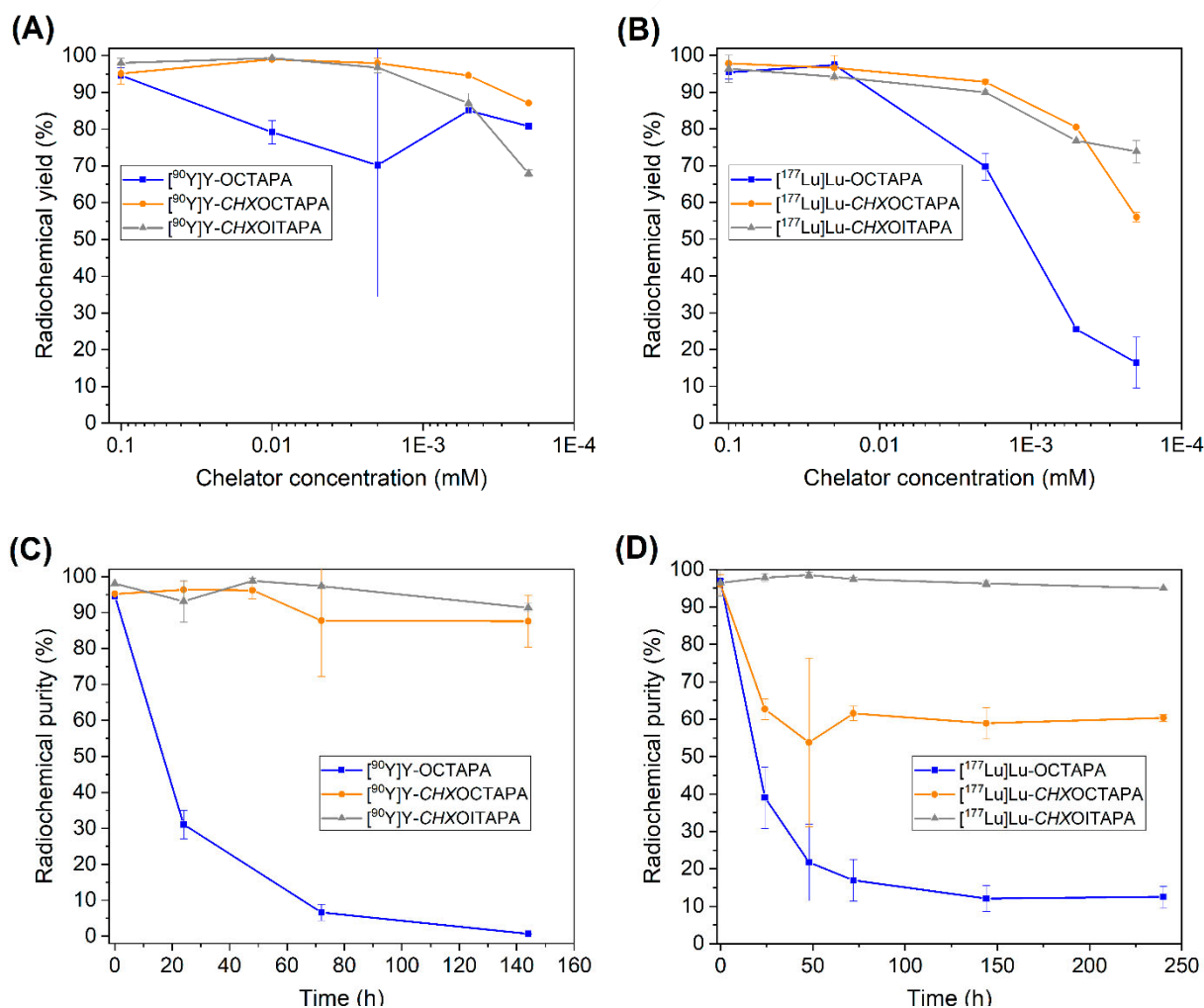
Figure 7. (A) and (B): Concentration-dependent radiolabeling of \text{H}_4\text{CHXOITAPA} , \text{H}_4\text{CHXOCTAPA} , and \text{H}_4\text{OCTAPA} with ^{90}\text{Y}^{3+} (10–50 MBq) (A) and ^{177}\text{Lu}^{3+} (20–40 MBq) (B), after 5 min reaction time at room temperature in \text{NH}_4\text{OAc} (10 mM, pH 5.5). (C) and (D): Stability (% intact complex remaining) measured at various time points after incubating the ^{90}\text{Y} - (C) and ^{177}\text{Lu} - (D) complexes of \text{CHXOITAPA}^{4-} , \text{CHXOCTAPA}^{4-} , and \text{OCTAPA}^{4-} in human serum at 37°C.
