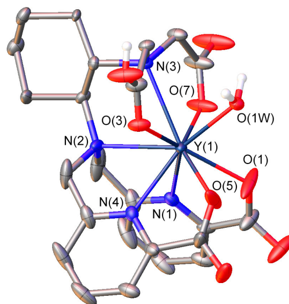
Figure 2. View of the X ray crystal structure of [Y(HCHXOITAPA)(H 2 O)] with 30% ellipsoid probability. Hydrogen atoms attached to C atoms, water molecules and the disorder of the cyclohexyl group were omitted for simplicity.
