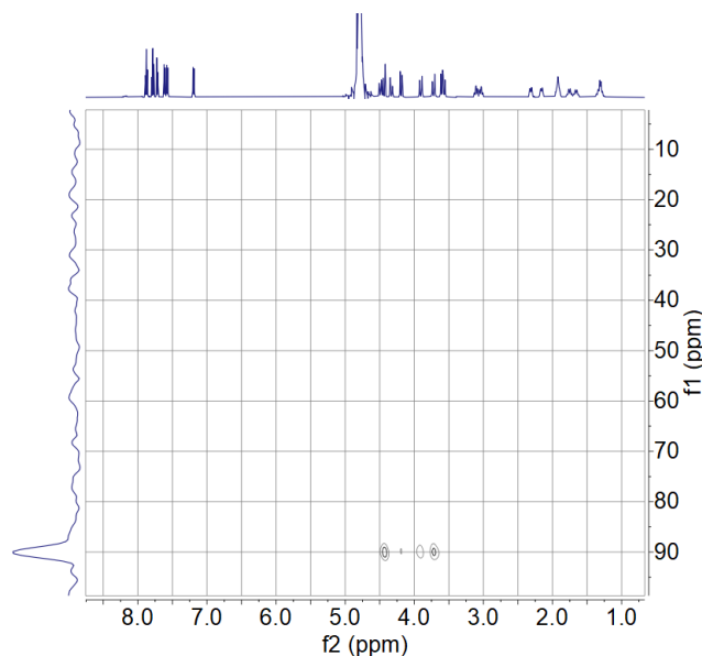
Figure 3. ^1H,^{89}Y -HMBC NMR spectrum of [Y(HCHXOITAPA)(H_2O)] recorded in D_2O solution (500 MHz, pH 6.84, 298 K).
