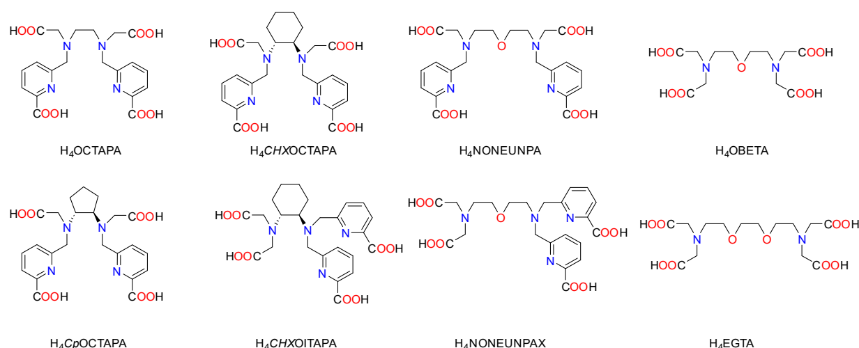
Figure 1. Structures of ligands discussed in the present work.
