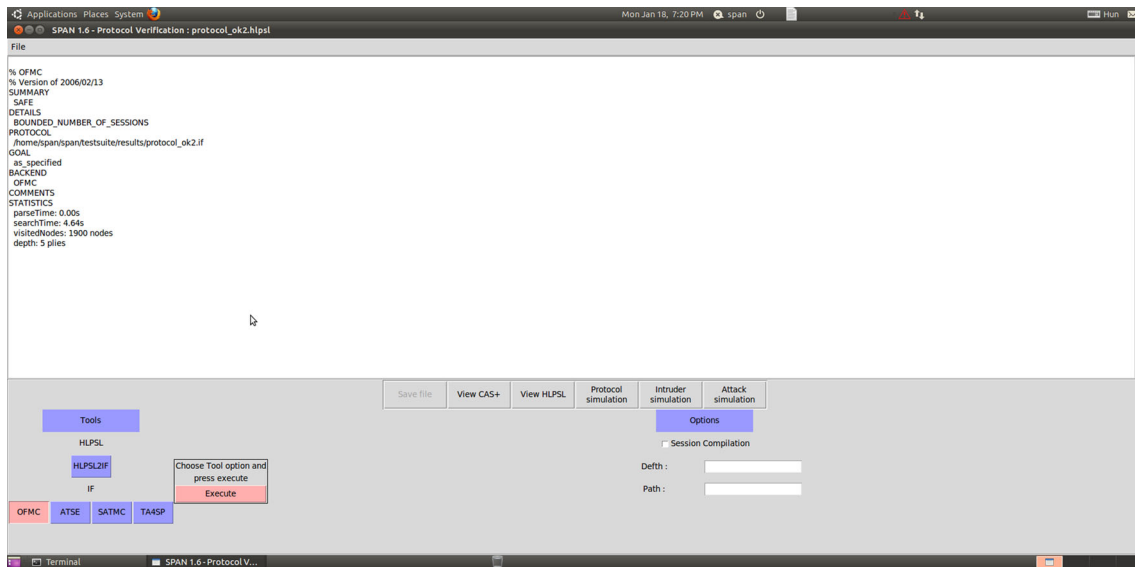
Fig. 11 OFMC output of the proposed protocol verified in AVISPA
