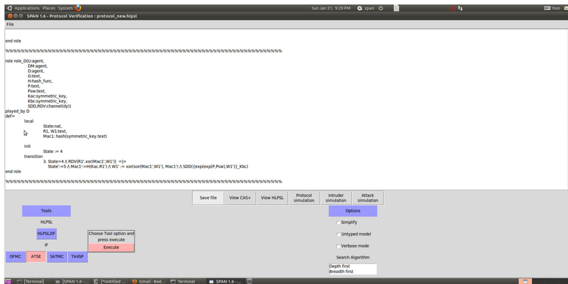
Fig. 9 HPSL specification of device's role
