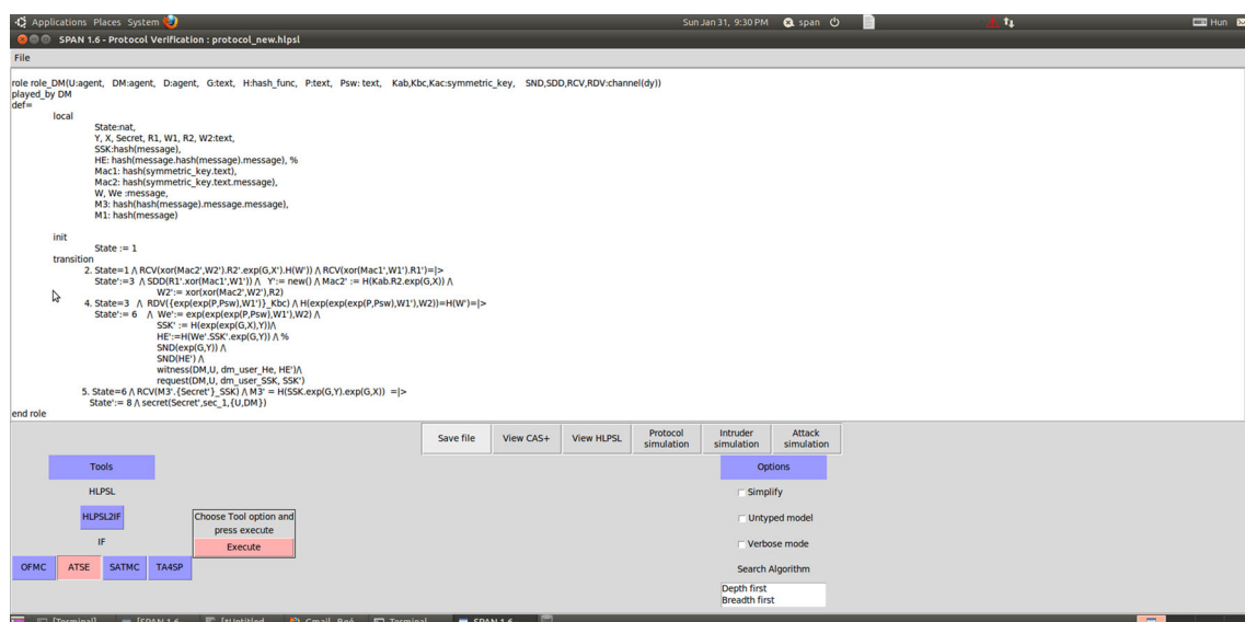
Fig. 8 HLPSSL specification of device manager's role
