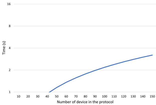
Fig. 5 Execution time for the client with different numbers of sensors
