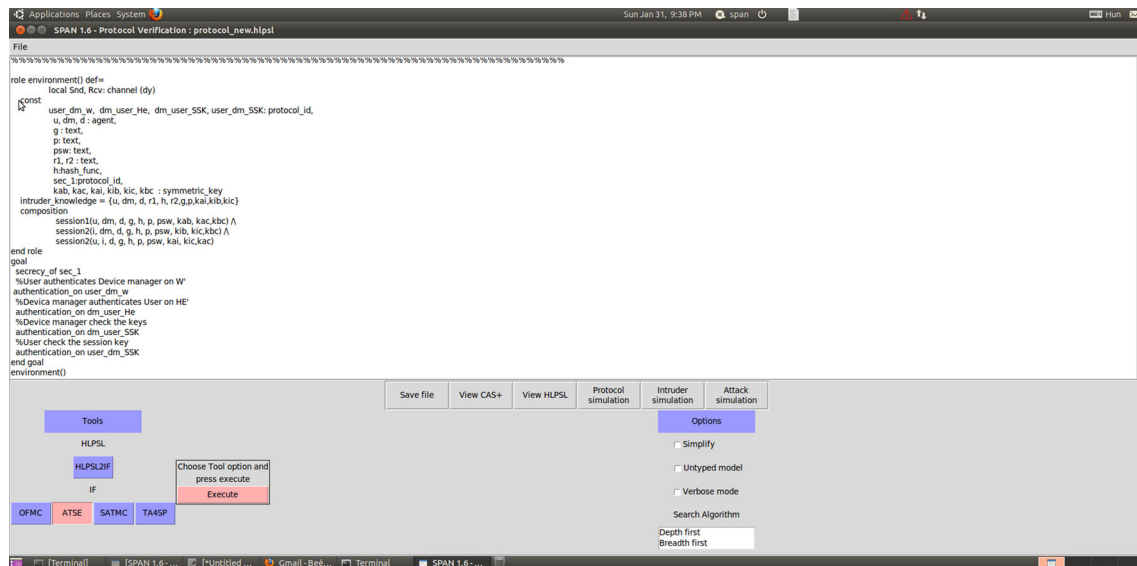
Fig. 10 HPSL Specification of role environment
