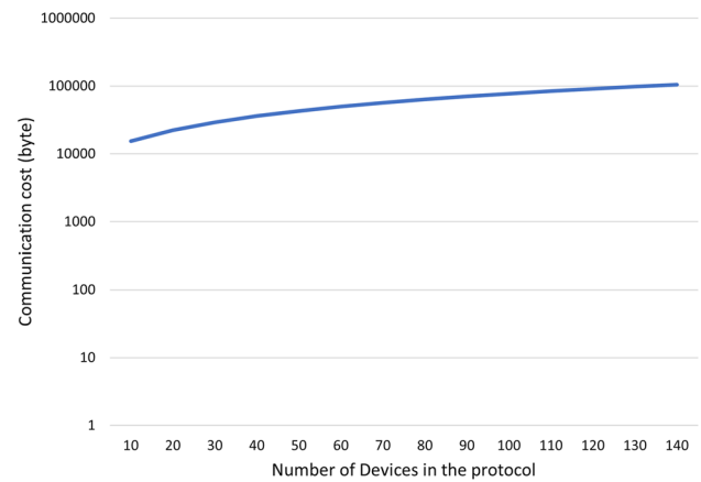
Fig. 6 Communication cost of the protocol with different numbers of sensors
