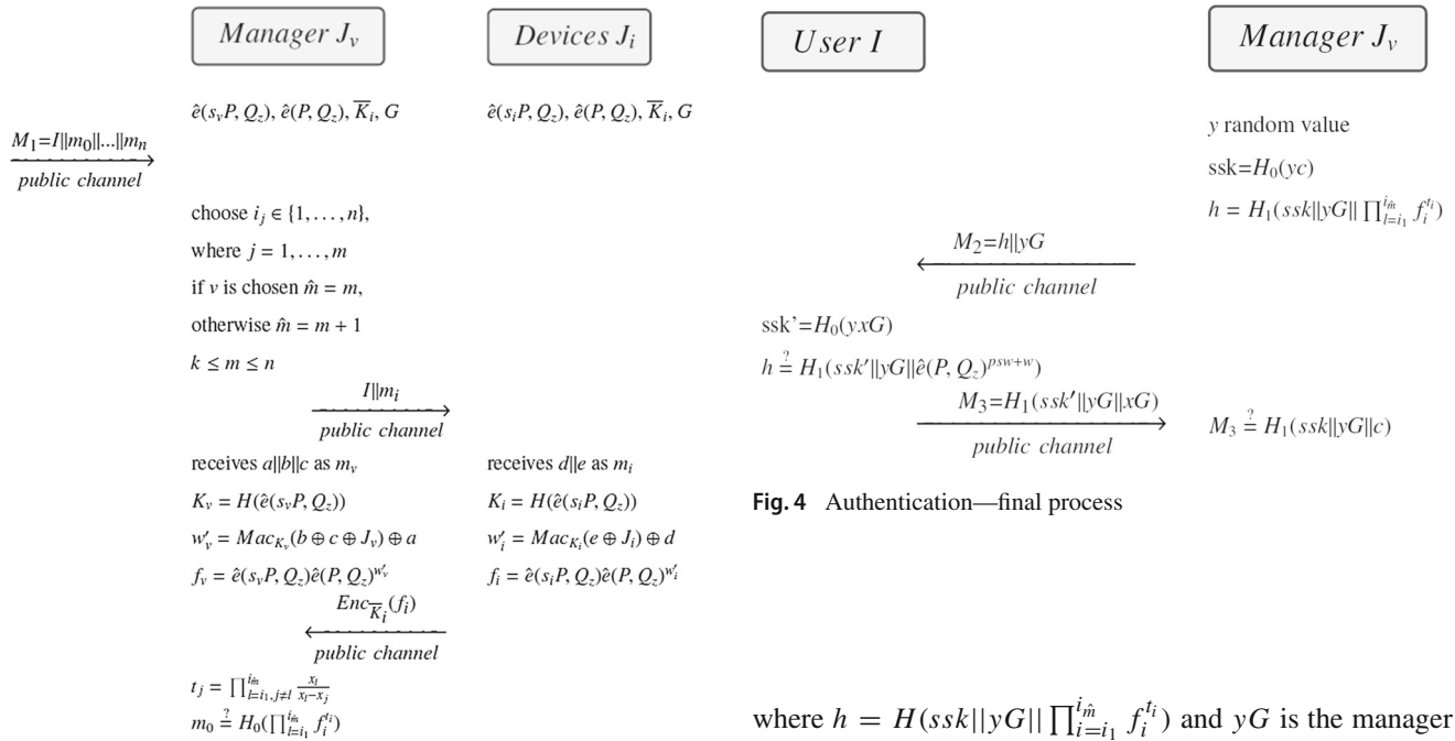
Fig. 3 Authentication—devices' process
