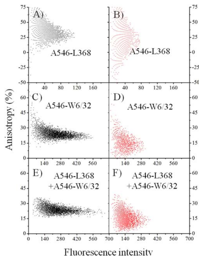
Fig. 7. Depolarized excitation speeds up intensity decay of anisotropies. The increased homo-FRET under depolarized excitation manifests itself also at the level of single cells, namely in the increased decay rates – “sensitization” – of the anisotropy vs. total intensity (i.e. dye concentration) curves. Shown are flow cytometric “anisotropy vs. total intensity” scatter plots (dot-plots) for the data of Fig. 5. Here anisotropy and intensity variations are supplied in a “natural way”, by the biological variance of the cells. In all panels anisotropies decrease with intensity at higher rates under depolarized illumination. Vertically polarized and depolarized excitations are illustrated with black and red dots, respectively. Panels A–D: “Anisotropy vs. total intensity” dot-plots for the A546-L368- and A546-W6/32-labeled samples. Panels E, F: “Anisotropy vs. total intensity” dot-plots for the A546-L368 + A546-W6/32 double-labeled homo-FRET sample.
