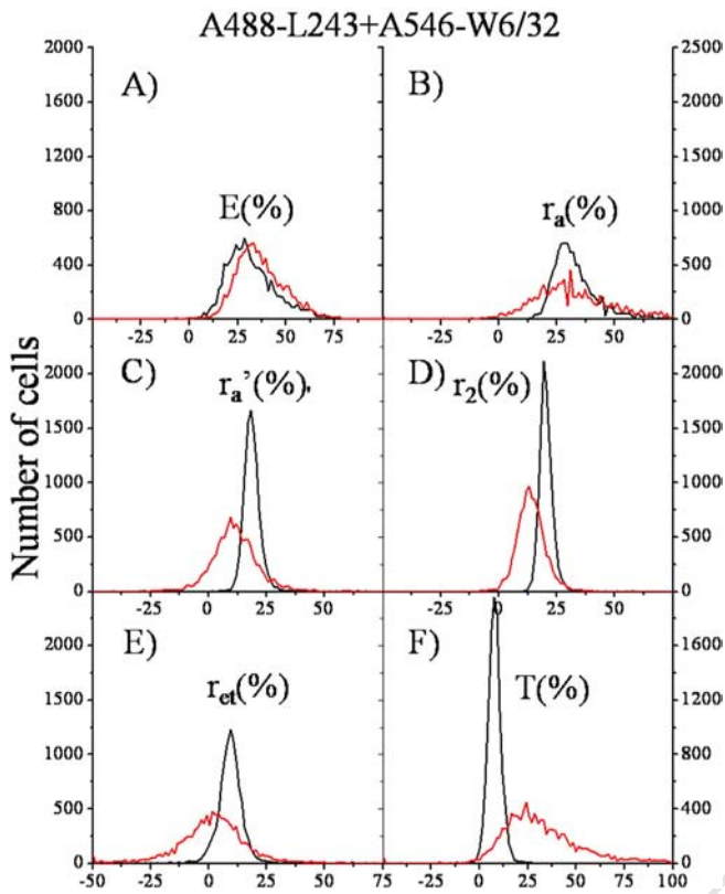
Fig. 4. FRET enhancement and FRET-mediated loss of acceptor anisotropy under depolarized excitation. Shown are representative flow cytometric polFRET histograms for the A488-L243 + A546-W6/32 mAb pair labeling the MHCII + MHC I h.c. receptor pair for excitation with vertically polarized and depolarized light, drawn with thin black and thick red lines, respectively. Depolarized excitation has been achieved by the Cornu#1-depolarizer in these experiments. Panel A: Conventional FRET efficiency E (Eq. (8)) is shifted to the right by excitation depolarization. Panel B: Anisotropy histograms measured for samples labeled only with acceptor ( r_a ) are practically located on the same mean with the two excitations. If anisotropy for the depolarized case would be computed the same way as for the polarized one, c.a. half the values should be obtained. r_a is a reference when FRET is assessed from acceptor anisotropy. Panel C: The relative decrease of acceptor anisotropy (Eq. (12)) measured in the presence of FRET r_a' as compared to its value without FRET, r_a is larger for depolarized excitation than for the polarized one, reinforcing the observation that depolarization enhances FRET efficiency E . Panel D: Another quantity, the directly measured anisotropy r_2 of the acceptor channel (Eq. (14)) can also be used for probing FRET. This is a more sensitive indicator than r_a' because it contains a contribution also from the donor anisotropy, in contrast to r_a' from which the contribution of donor is separated. Although, r_2 is properly referenced to the average anisotropy of the donor and acceptor both measured in the acceptor channel (Eq. (13), not indicated), as an approximation it can also be referenced to the pure acceptor anisotropy r_a , because the donor contribution is generally small. Panel E: Reduction in anisotropy of sensitized emission under depolarized excitation. Anisotropy of sensitized emission of acceptor, r_{et} (Eq. (11)) which is not zero for polarized excitation – albeit it is much smaller than that of direct emission, r_a – has been reduced to zero under depolarized excitation. That for polarized excitation the anisotropy of sensitized emission is not zero is a direct proof for that the relative orientation of the donor and acceptor is not random for this donor–acceptor pair. In contrast, under depolarized excitation the zero r_{et} means that the relative orientation is randomized leading to new FRET pathways, and consequently, enhanced FRET efficiency. Panel F: Increased “polarized FRET efficiency” T under depolarized excitation. Another way for the joint description of FRET efficiency and the anisotropy of sensitized emission is via the “polarized FRET efficiency” T . This quantity can be obtained by expressing the FRET efficiency E from Eqs. (13) and (14) as functions of the measurable anisotropy ratios either r_a'/r_a or r_2/r_{2,av} and with the anisotropy of sensitized emission as an assumed input constant. The two measures of FRET, E and T , coincide whenever r_{et} is zero. Otherwise, possible deviations of r_{et} from zero are transformed into corresponding deviations of T and E : T underestimates E for positive r_{et} and upper-estimates it for negative r_{et} . While for polarized excitation T is smaller than E , indicating that r_{et} is not zero, for depolarized excitation T is close to E , indicating a vanishing r_{et} .
