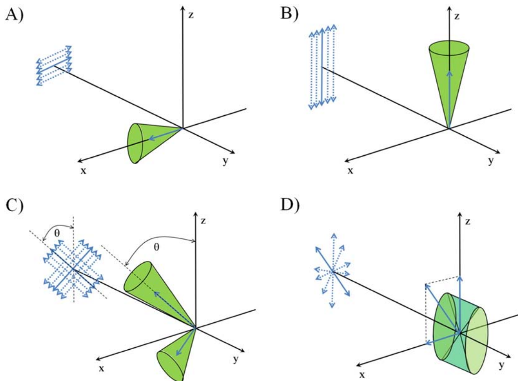
Fig. 3. Modes of photoselection. In all panels the traveling direction of the exciting light is in the direction of the y axis, the observation is along the x axis. Panel A: Horizontally polarized light is used for determining the G-factors, which is used for calculation of anisotropies in the other excitation modes. The photoselected dipoles constitute a cone (green) with the observation direction (x), as the axis of symmetry. In reality there exists another cone in the direction of the (−x) axis, but this is omitted for simplicity. Panel B: Vertically polarized light is used for calculating the emission anisotropy and total intensity of the fluorophores. These quantities can be taken as molecular attributes which are independent from the mode of photoselection, and they should be given back also by the other excitation modes. Panel C: Diagonally polarized excitation, as a combination of the previous horizontal and vertical ones, rotated by an arbitrary angle \theta from the vertical (z) direction. The photoselected dipole ensemble is the superposition of those for the horizontal and vertical polarizations. It can be shown, that the way of calculation of the anisotropy is the same as for the depolarized excitation, independently from \theta (see at the end of Supporting information ). Panel D: Depolarized excitation. Formally it can be obtained from the previous polarized and diagonally polarized cases by random rotations of the photon field vectors (blue double arrows) from their original directions in the x–z plane. Consequently the photoselected ensemble can be obtained by rotating the corresponding cones around the y axis. The photoselected ensemble constitute a volume also obtainable from the sphere representing all spatial orientations – the total 4\pi steric angle – by omitting two conical volumes around the (+y) and (−y) axes [24,25]. An alternative construction of the photoselected ensemble is by making the horizontal and vertical projections for each field vector and taking into account the corresponding cones with the squares of the projections as intensity weights (see in Supporting information ). Rotation of polarization direction has been achieved with a Fresnel double-rhomb, depolarization with Cornu#1 and Cornu #2 depolarizers or with a circular polarizer, diagonal polarization by a polarizing parallel beam-splitter.
