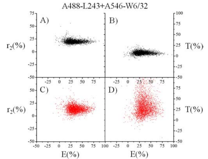
Fig. 5. Excitation depolarization sensitizes FRET dependence of the combined anisotropy r_{2,av} and the “polFRET efficiency” T . Shown are representative flow cytometric polFRET dot-plots for the data of Fig. 3 – i.e., for the A488-L243 + A546-W6/32 mAb pair – for excitation with vertically polarized and depolarized light, drawn with black and red dots, respectively. Panels A, B: For vertically polarized excitation both the anisotropy r_2 (Panel A) and “polFRET efficiency” T (Panel B) depend only weakly on the conventional FRET efficiency E . Panels C, D: For depolarized excitation both the anisotropy r_2 (Panel C) and “polFRET efficiency” T (Panel D) depend rather strongly on the conventional FRET efficiency E . The stronger dependence can be attributed to the observation that sensitized emission is totally depolarized under depolarized excitation as compared to the polarized one.
