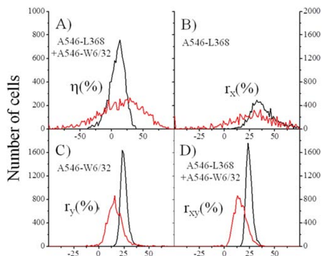
Fig. 6. Increased homo-FRET under depolarized excitation. Homo-FRET has been quantified by the relative decrease of anisotropy of the sample labeled with both the A546-L368 and A546-W6/32 mAbs as compared to the intensity-weighted average of the anisotropies for the corresponding singly-labeled samples (Eqs. 12s, 13s Supporting information). Because both mAbs bind to the same MHC molecule, large proximity of mAbs, and as a result, high homo-FRET can be expected in this case. Vertical polarization is illustrated with thin black line, depolarized one – realized with the Cornu#1 depolarizer – with thick red line. Panel A: Flow cytometric histogram of homo-FRET enhancement ( \eta ) obtained in the depolarized light is shifted to the right as compared to the one in vertically polarized light, reporting on a substantial homo-FRET increase. The increase in homo-FRET, similarly to the case of hetero-FRET, is expected due to the more favorable mutual orientations of the donor – the primarily photo-excited dyes – and acceptor dipoles in depolarized illumination. Panel B: Anisotropy histograms for the A546-L368-labeled sample, necessary for the computation of the reference average anisotropy. The mean values obtained with the two polarization modes are almost the same, as expected, however the widths of the curves are substantially different. The slight differences in the mean anisotropies can be attributed partly to possible optical path differences between the polarization modes described by different G-factors and/or aperture depolarization factors – the a(\psi) -factor in the formulae for total intensity, Eqs. (2) and (4), partly to a homo-FRET increase even on the singly-labeled samples. The larger histogram widths belonging to the depolarized case can be attributed to the intensity loss in the depolarizer. Panel C: Anisotropy histograms for the A546-W6/32-labeled sample, the other component for the average anisotropy. Panel D: Anisotropy histograms for the homo-FRET sample, double-labeled with the A546-L368 and A546-W6/32 mAbs, from which with referencing to the corresponding averages the homo-FRET enhancement curves on Panel A have been deduced. Although both histograms are shifted to the left of the corresponding averages indicating that homo-FRET is present in both excitation modes, the larger shift belongs to the depolarized mode indicating that homo-FRET is larger in this mode.
