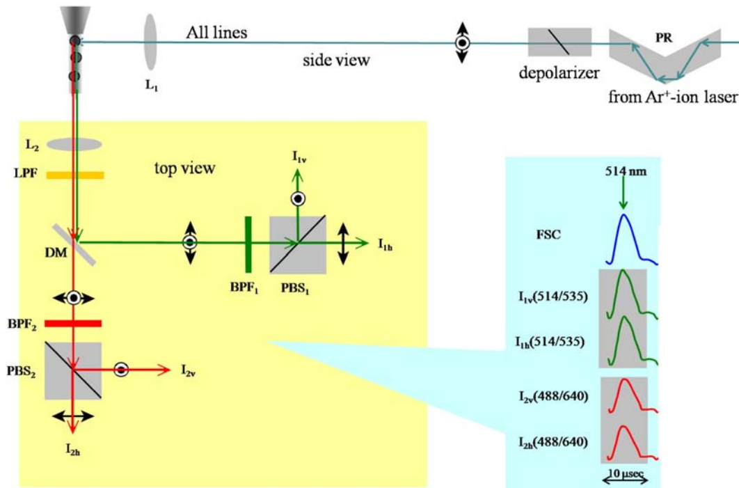
Fig. 2. Optical layout of single-laser polFRET and detected signals. The beam of an Ar + -laser in “all-lines” mode is fed into the cytometer through a “Fresnel double-rhomb” polarization rotator (PR) onto which a depolarizer – Cornu, quarter-wave plate, parallel beam-slit – is mounted. The fluorescence is collected by a lens (L 2 ), directed after the long-path filter (LPF) by a dichroic mirror beam-splitter (DM) towards the polarization beam-splitter cubes (PBS 1 , PBS 2 ), which together with the respective band-pass filters (BPF 1 , BPF 2 ) constitute the “green (#1)” and “red (#2)” polarized intensity channels.
