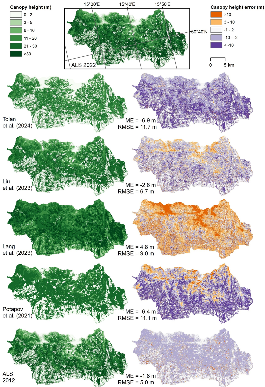
Figure 2. Canopy heights from four predicted canopy height maps from spaceborne LiDAR: Tolan et al. (2024), Liu et al. (2023), Lang et al. (2023), and Potapov et al. (2021) and an outdated (2012) ALS compared with a recent (2022) ALS model (reference data set). The figures on the left show canopy height, while the figures on the right show the difference in canopy height compared to the ALS 2022 data (i.e., the error of the predicted maps). ME stands for mean error, and RMSE stands for root mean square error.
