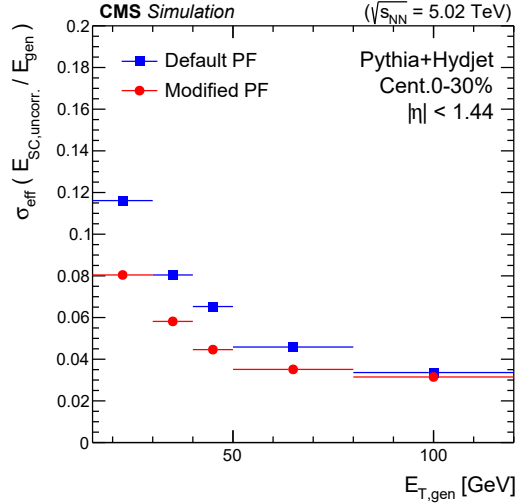
Figure 36. Photon energy resolution comparison in simulation for different PF clustering algorithms in PbPb collisions as a function of the generated photon E_{\text{T}} . The default algorithm (in blue) has a dynamic \eta - \phi window, and is compared to the modified PF clustering algorithm with an upper bound on the SC extent in the \phi direction (in red). Barrel photons ( |\eta| < 1.44 ) are used in simulated PbPb events within the 0–30% centrality range.
