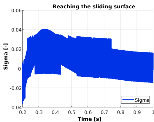
Figure 10: After reaching the sliding surface, the sliding mode becomes active.
