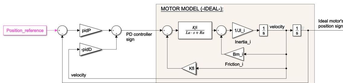
Figure 5: Model of the ideal motor with the application of a PD controller.
