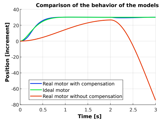
Figure 15: An additional load added to the system.
