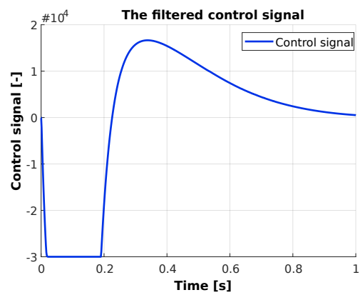
Figure 12: The filtered signal of the sliding-mode controller.
