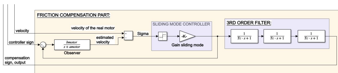
Figure 6: The component with regard to the compensation of friction.
