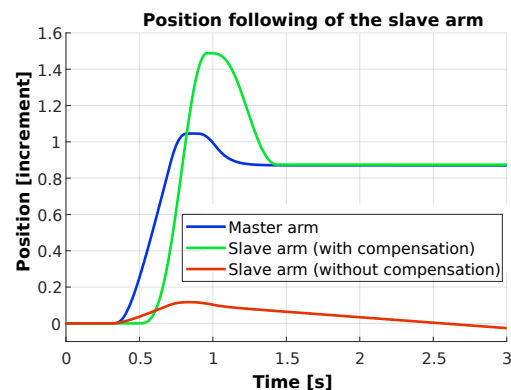
Figure 18: Position signal following of the bilateral system.
