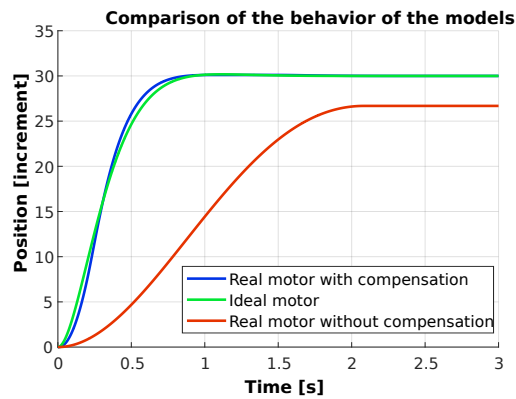
Figure 14: Position signals after Coulomb friction was accounted for in the system.
