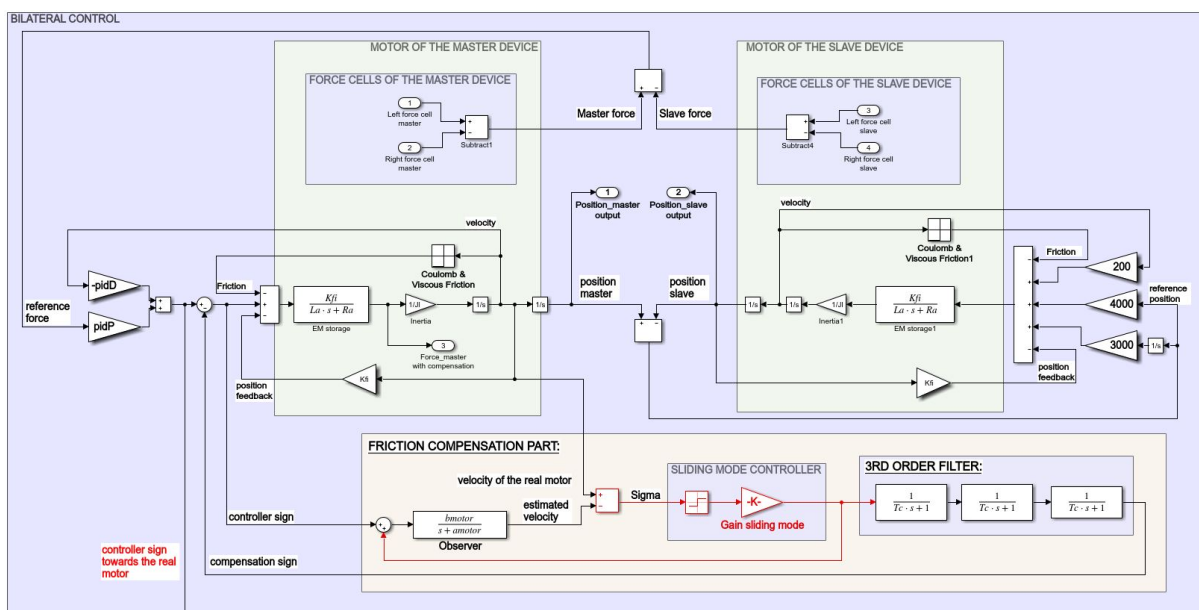
Figure 16: Bilateral control model.
