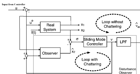
Figure 1: Sliding mode-based disturbance compensation.
