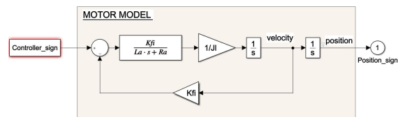
Figure 3: Model of the master and slave devices.
