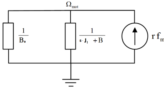
Figure 4: Model of the feedback force.
