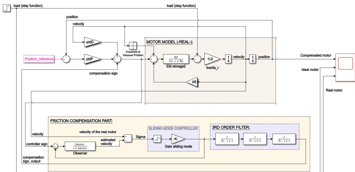
Figure 13: Full model of the compensated motor subjected to calibration.
