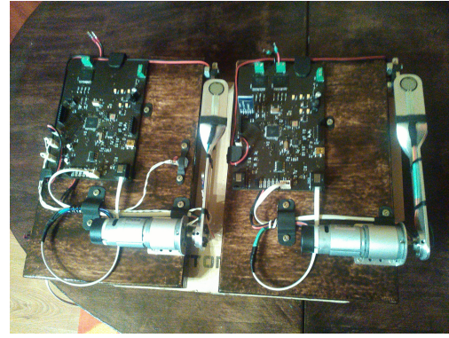
Figure 2: The haptic device.
