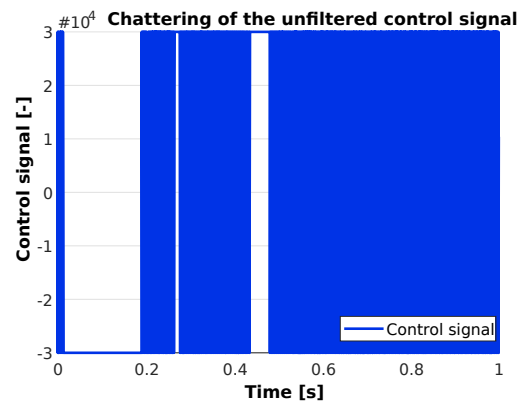
Figure 11: Chattering originating from the output of the sliding-mode controller.
