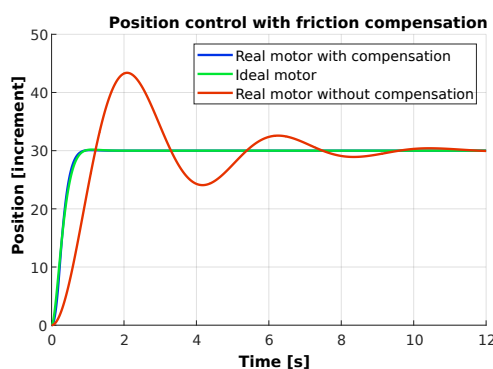
Figure 7: The compensated signal follows the stated trajectory.
