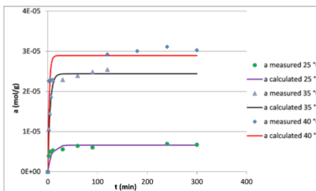
Fig. 5 Arsenite (III) sorption kinetics at 25^\circ \text{C} , 35^\circ \text{C} and 40^\circ \text{C} on lanthanum modified bentonite, 100 mg bentonite, 20 \text{ cm}^3 5 \times 10^{-4} \text{ mol dm}^{-3} \text{ Na}_3\text{AsO}_3 , pH 7.0-8.43
