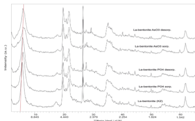
Fig. 7 XRD spectrum of La-bentonite and that of after sorption and desorption of arsenite and phosphate, the unit of y axis is arbitrary unit (a.u.)
